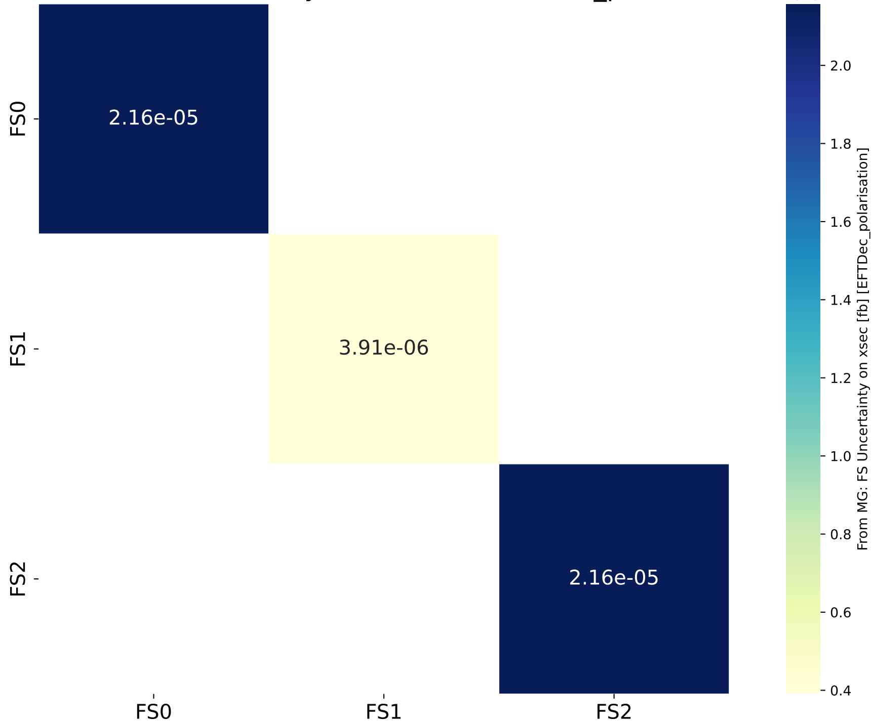
From MG: FS Uncertainty on xsec [fb] [EFTDec_polarisation]
