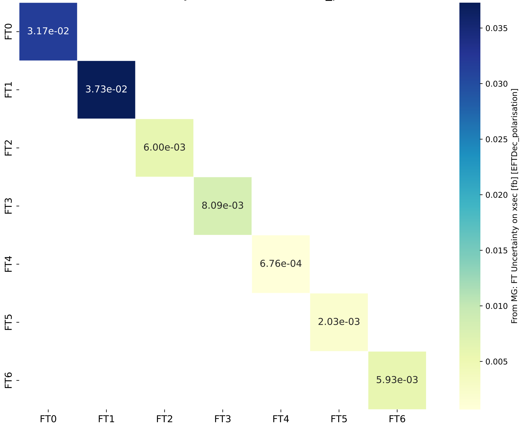
From MG: FT Uncertainty on xsec [fb] [EFTDec_polarisation]
