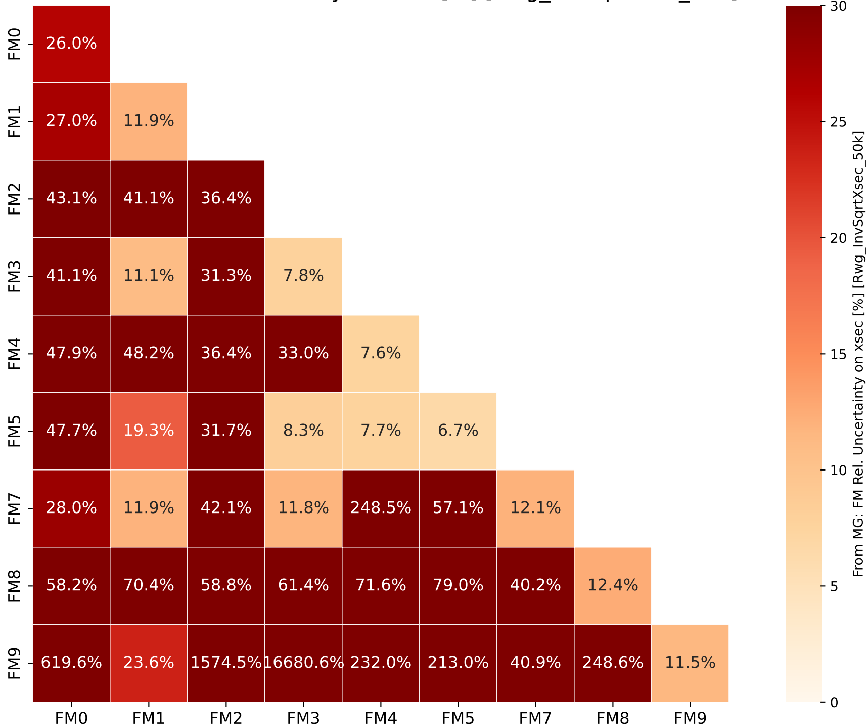
From MG: FM Rel. Uncertainty on xsec [%] [Rwg_InvSqrtXsec_50k]
