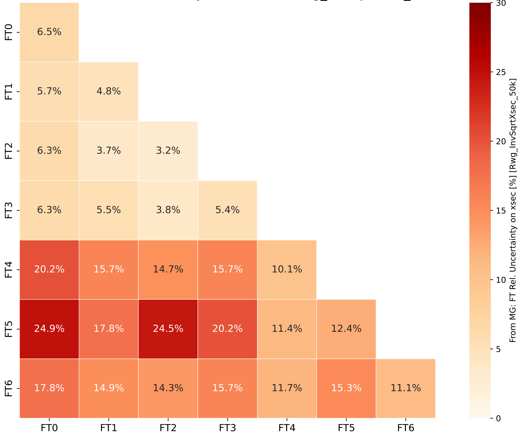
From MG: FT Rel. Uncertainty on xsec [%] [Rwg_InvSqrtXsec_50k]
