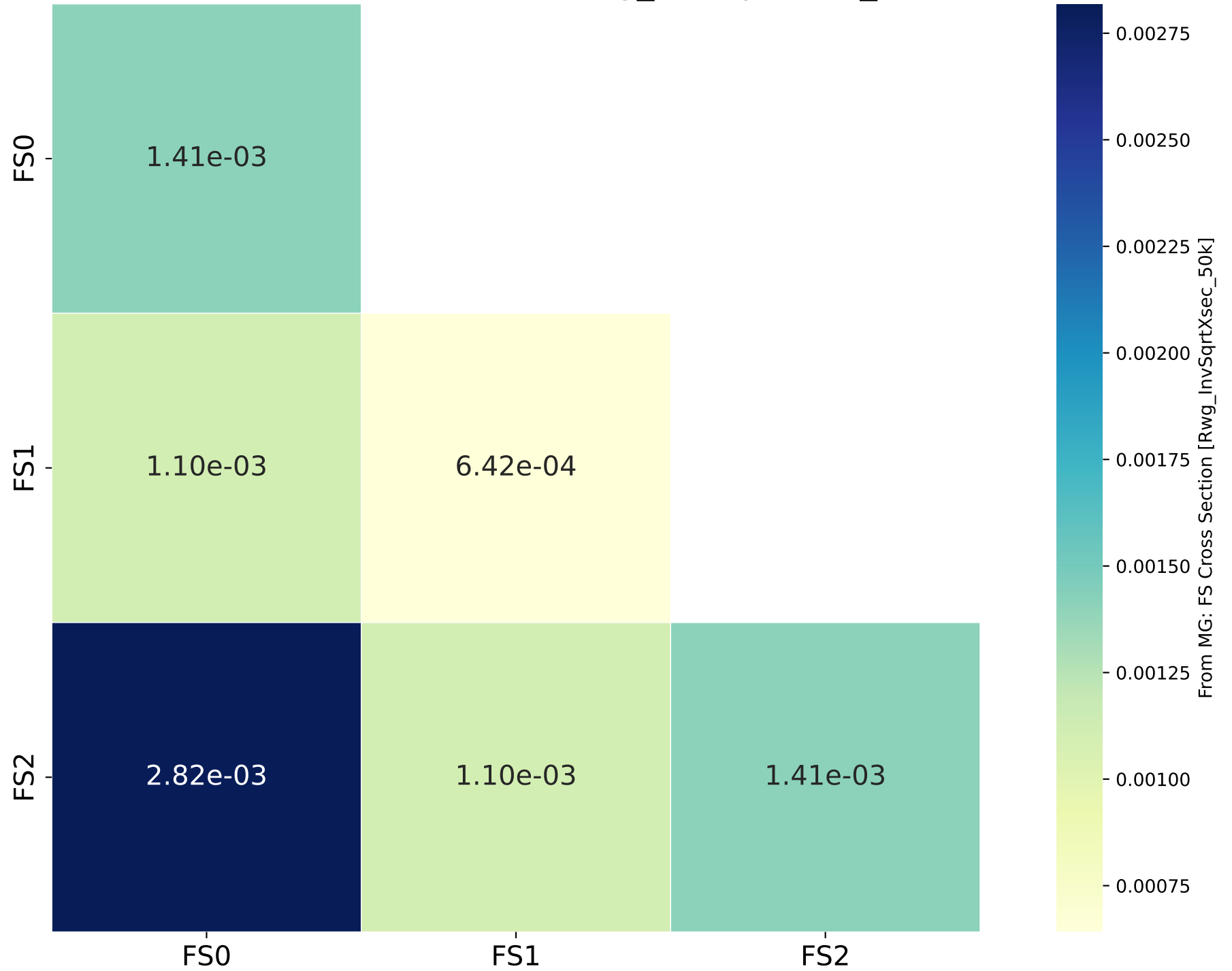
From MG: FS Cross Section [Rwg_InvSqrtXsec_50k]
