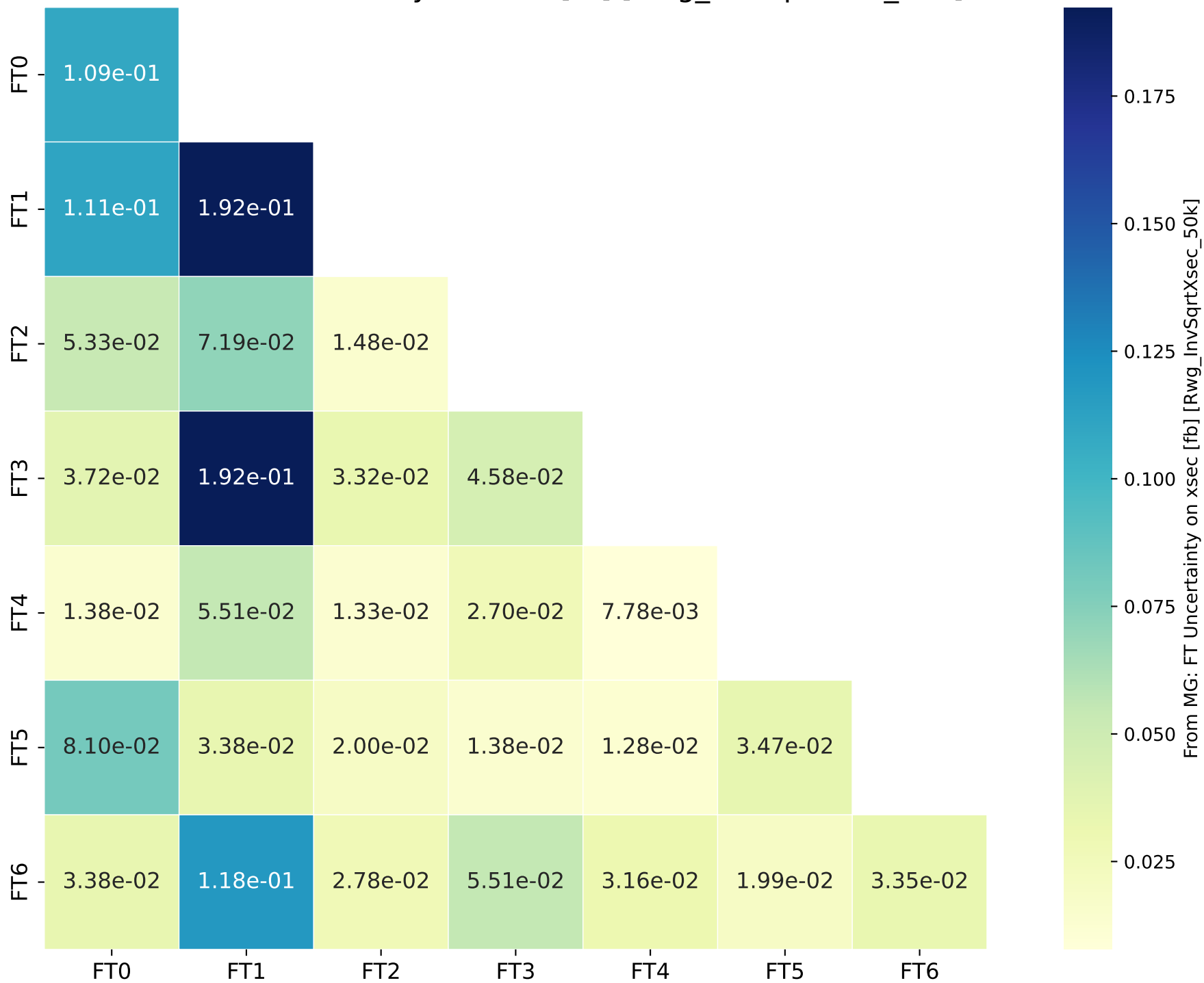
From MG: FT Uncertainty on xsec [fb] [Rwg_InvSqrtXsec_50k]
