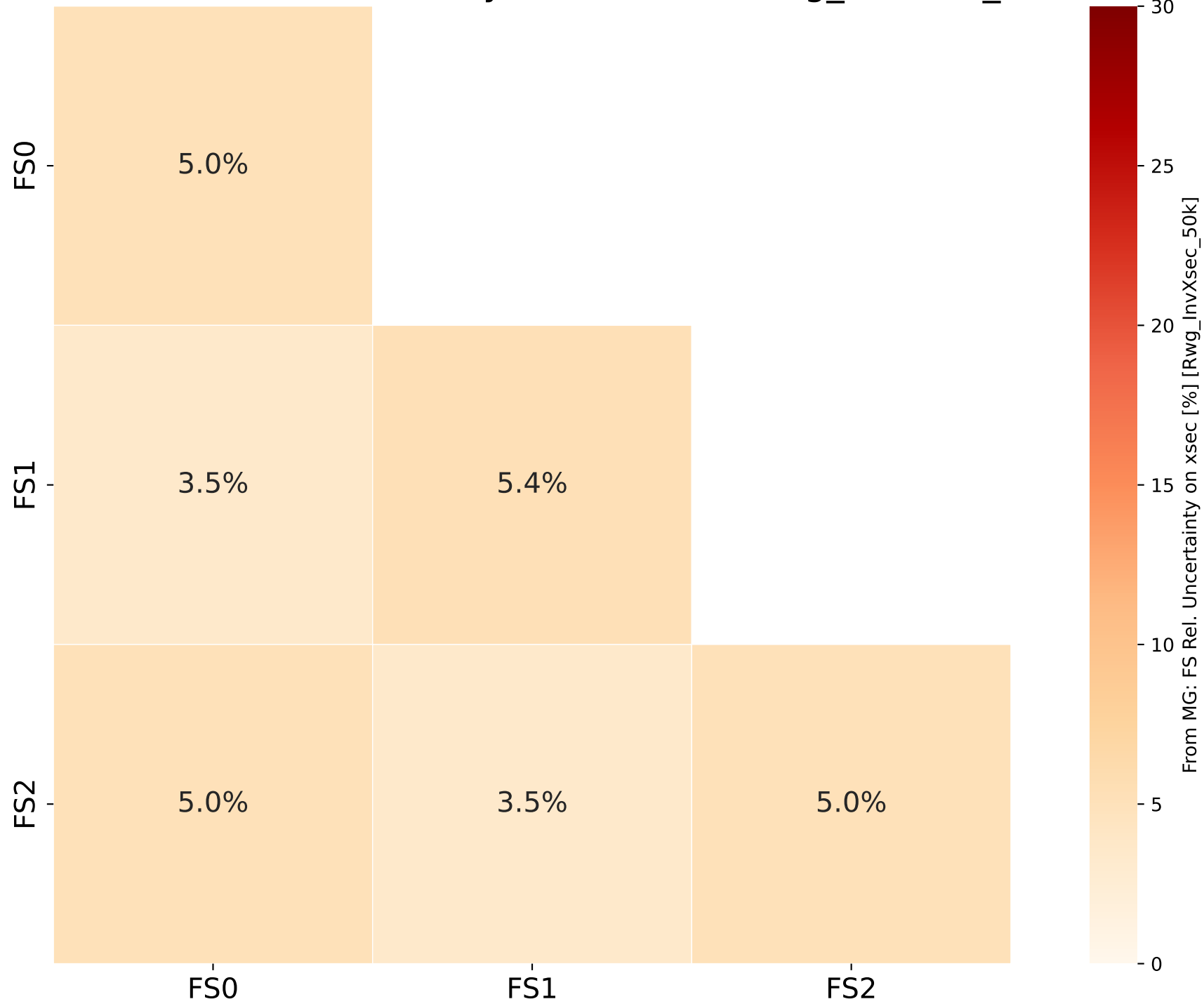
From MG: FS Rel. Uncertainty on xsec [%] [Rwg_InvXsec_50k]
