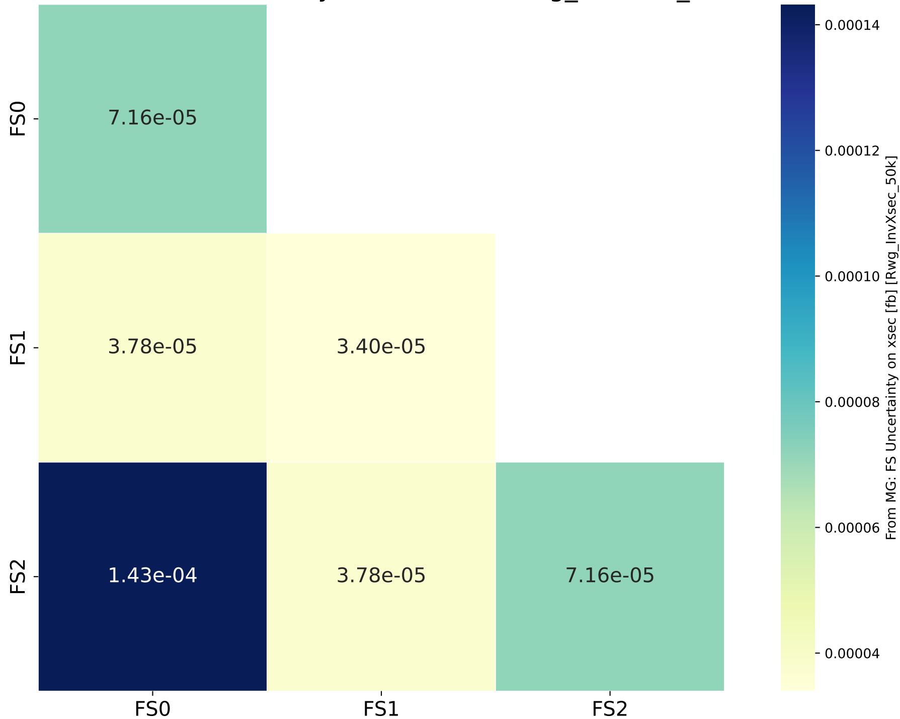
From MG: FS Uncertainty on xsec [fb] [Rwg_InvXsec_50k]
