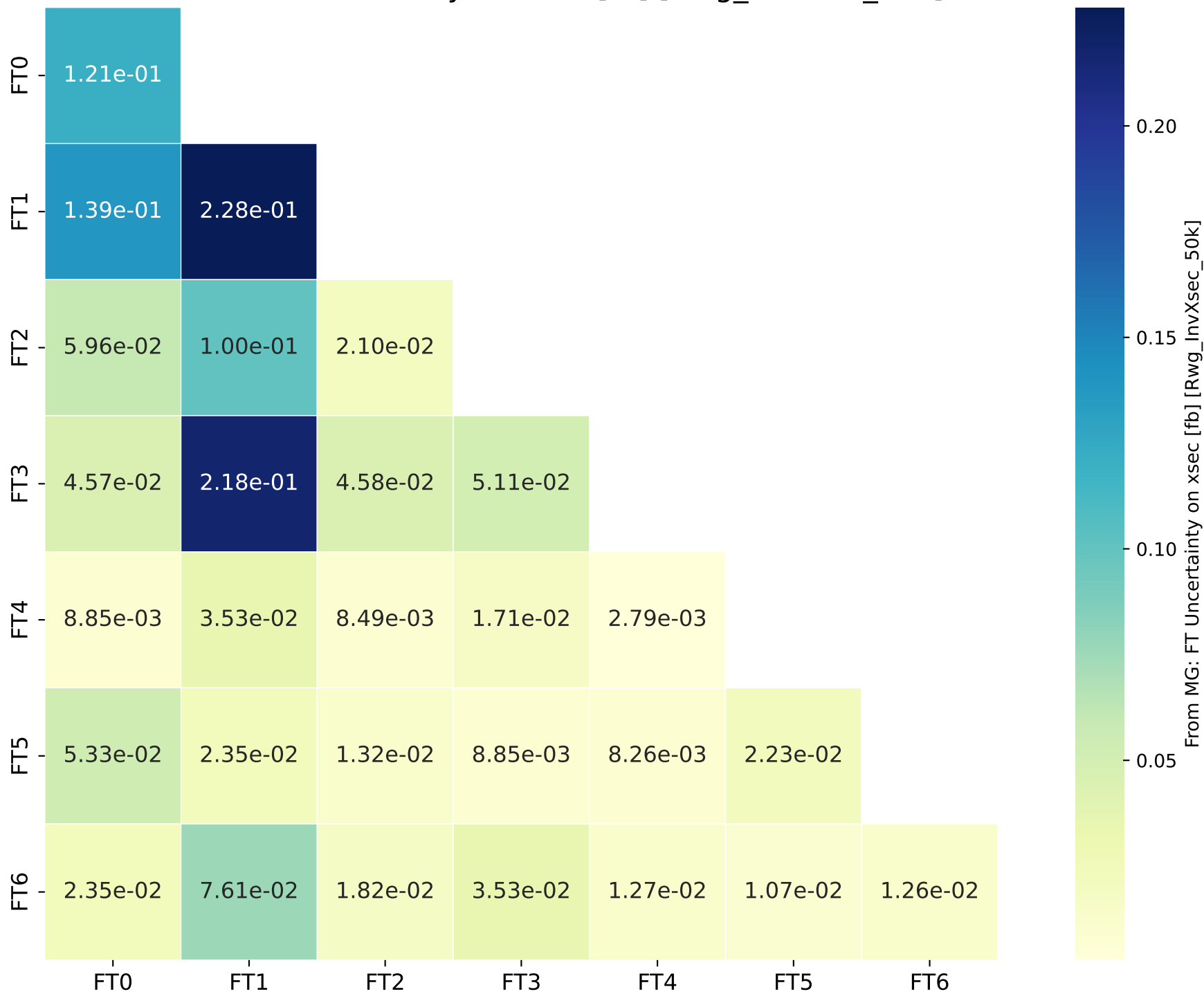
From MG: FT Uncertainty on xsec [fb] [Rwg_InvXsec_50k]
