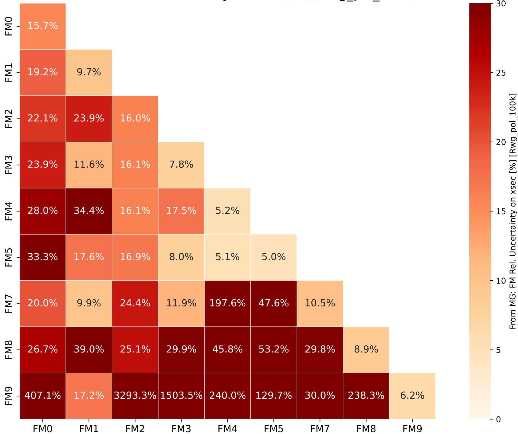
From MG: FM Rel. Uncertainty on xsec [%] [Rwg_pol_100k]
