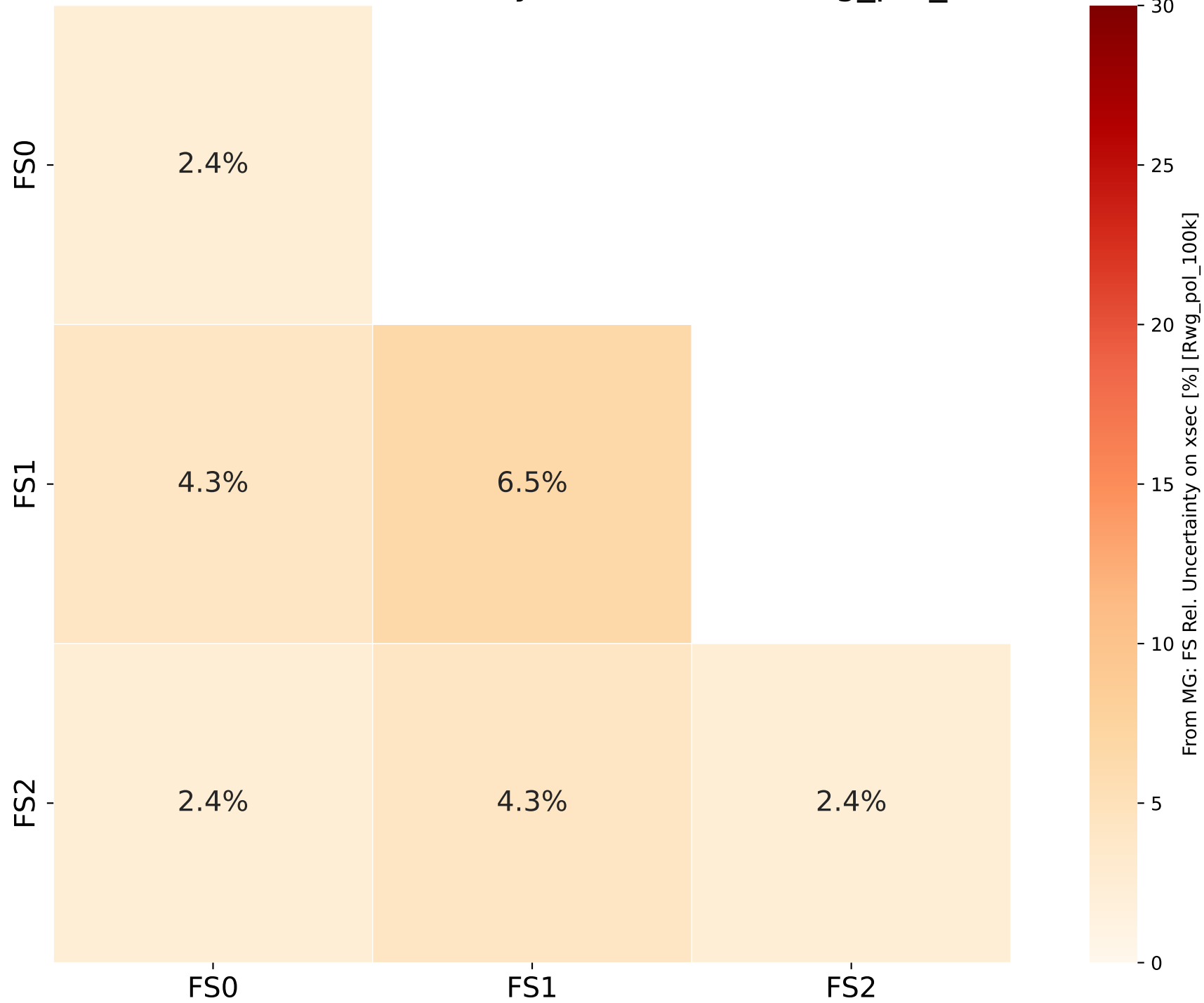
From MG: FS Rel. Uncertainty on xsec [%] [Rwg_pol_100k]
