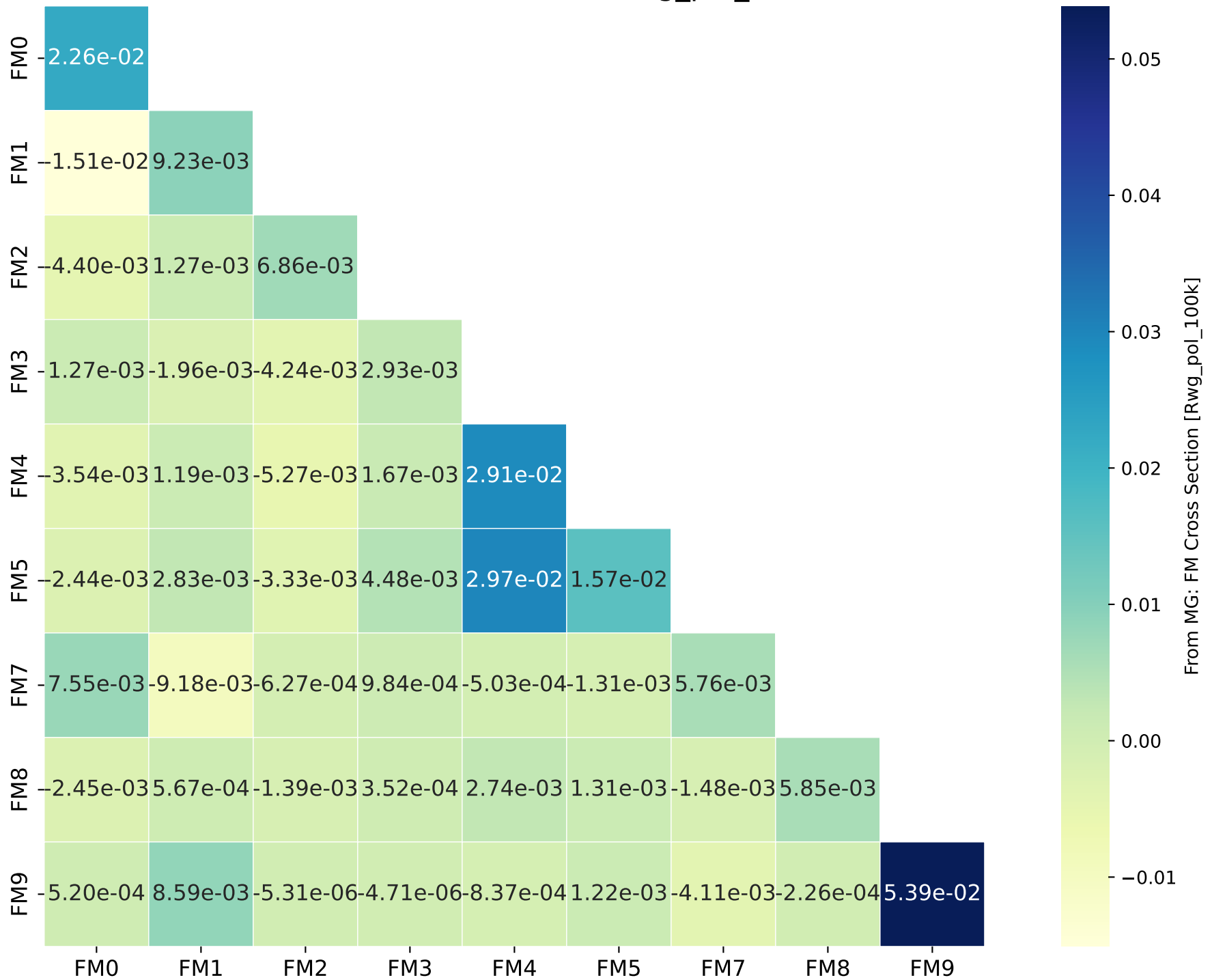
From MG: FM Cross Section [Rwg_pol_100k]
