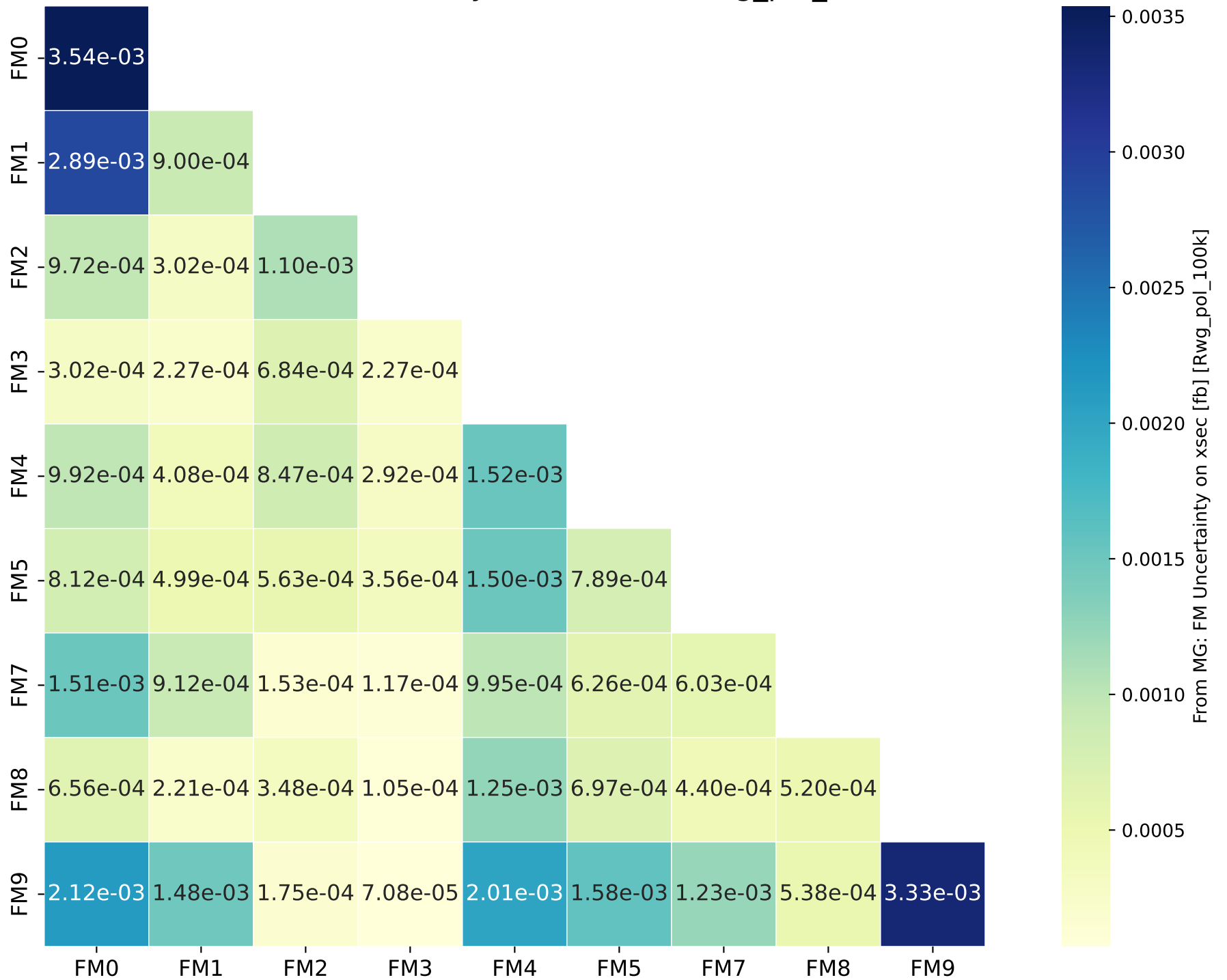
From MG: FM Uncertainty on xsec [fb] [Rwg_pol_100k]
