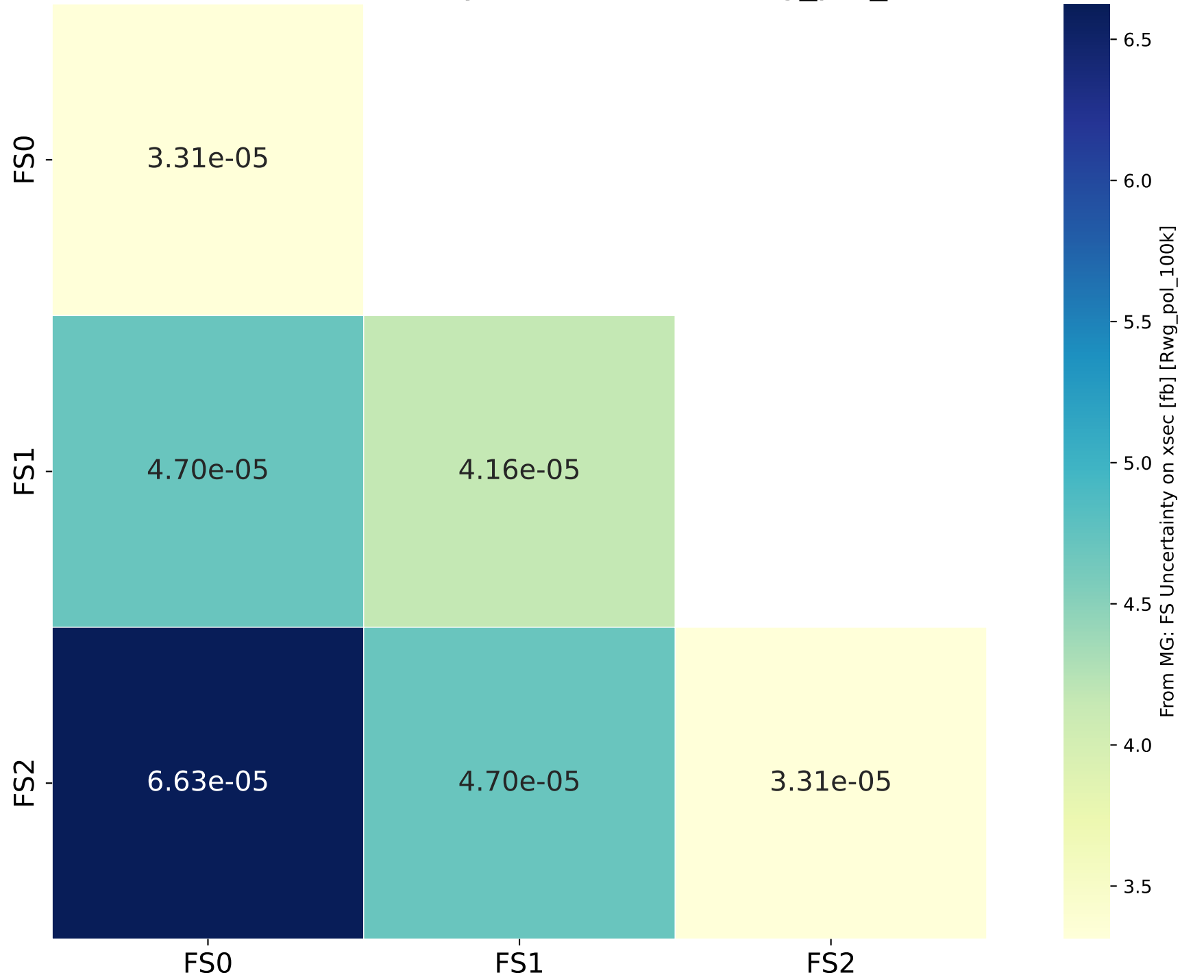
From MG: FS Uncertainty on xsec [fb] [Rwg_pol_100k]
