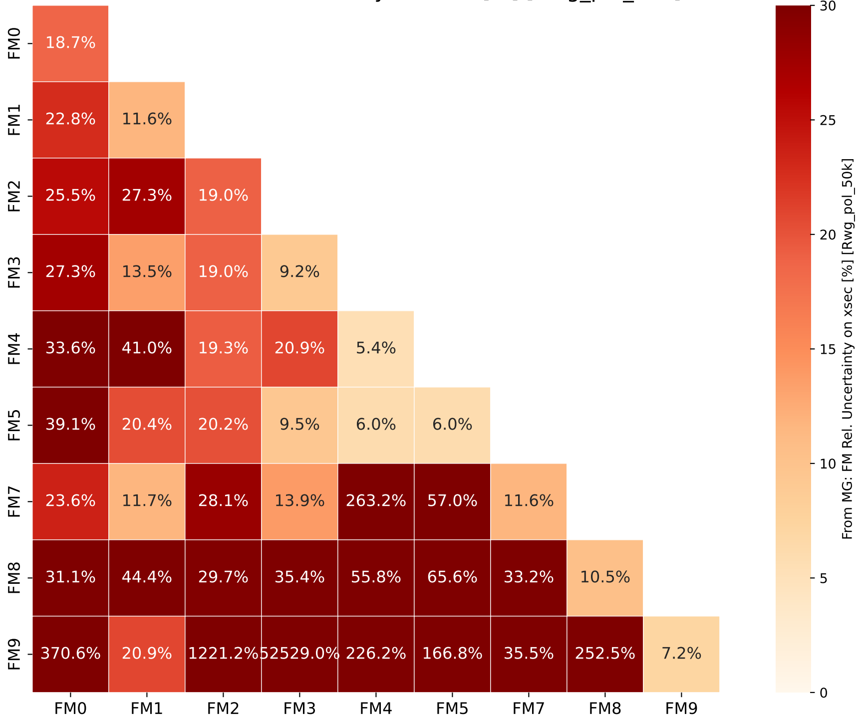
From MG: FM Rel. Uncertainty on xsec [%] [Rwg_pol_50k]
