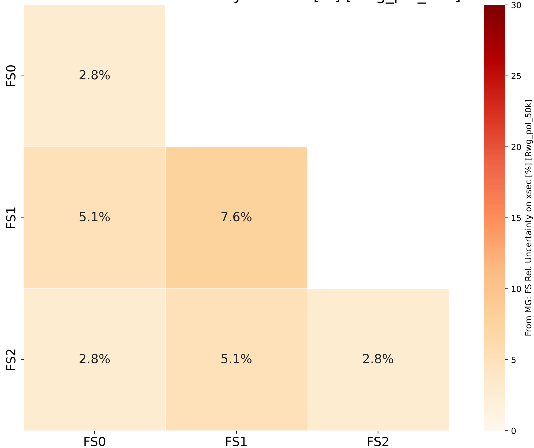
From MG: FS Rel. Uncertainty on xsec [%] [Rwg_pol_50k]
