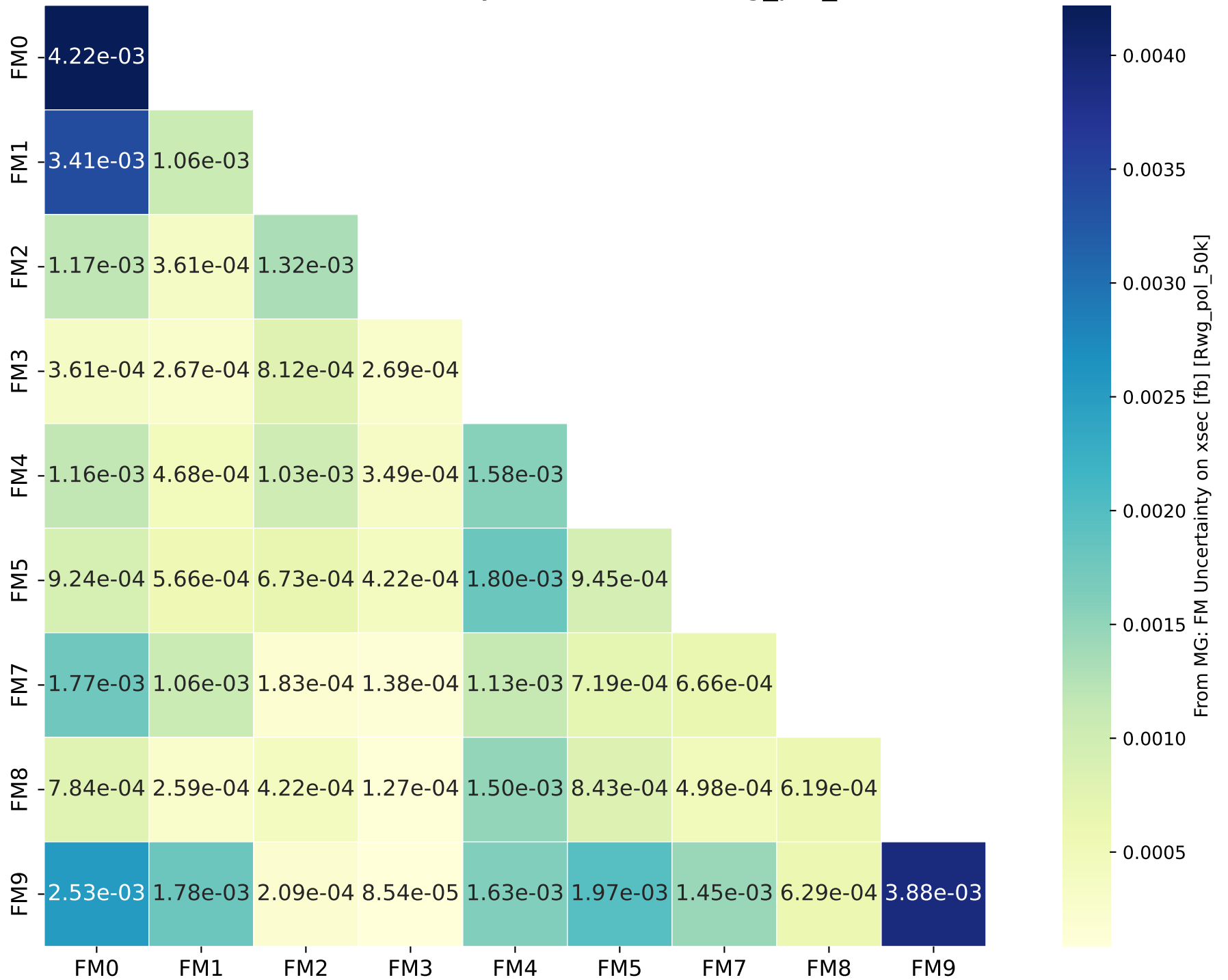
From MG: FM Uncertainty on xsec [fb] [Rwg_pol_50k]
