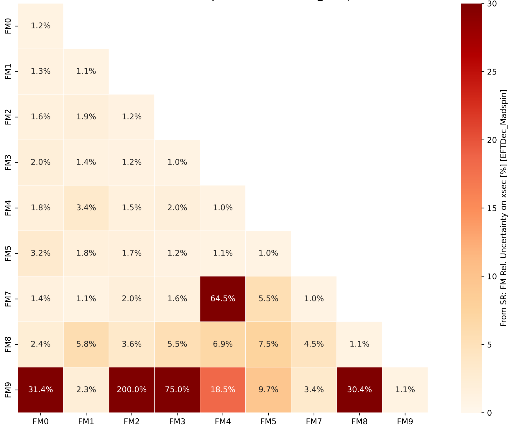
From SR: FM Rel. Uncertainty on xsec [%] [EFTDec_Madspin]
