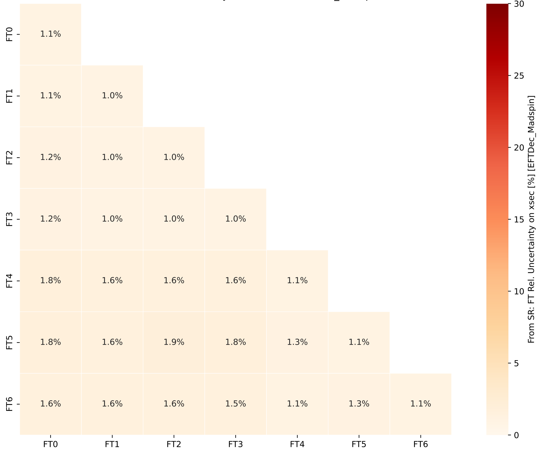
From SR: FT Rel. Uncertainty on xsec [%] [EFTDec_Madspin]
