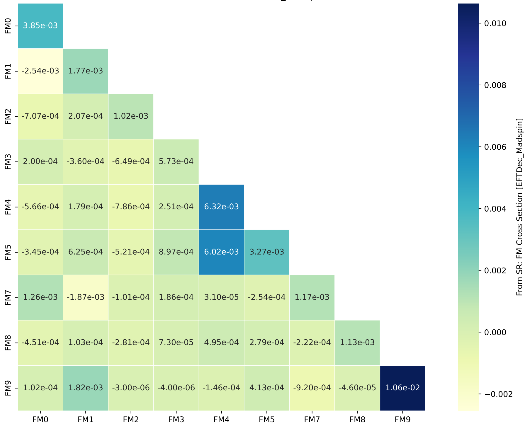
From SR: FM Cross Section [EFTDec_Madspin]
