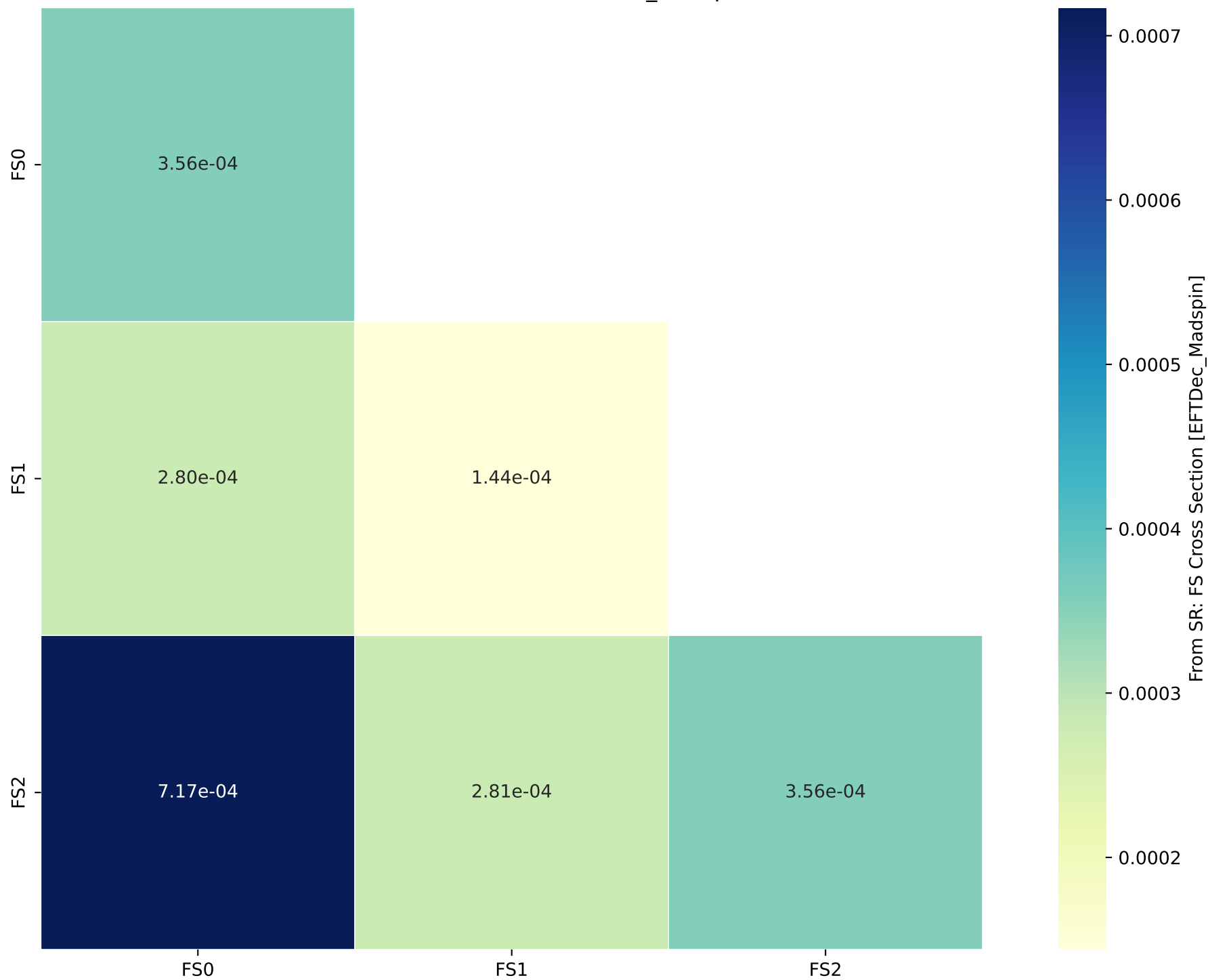
From SR: FS Cross Section [EFTDec_Madspin]
