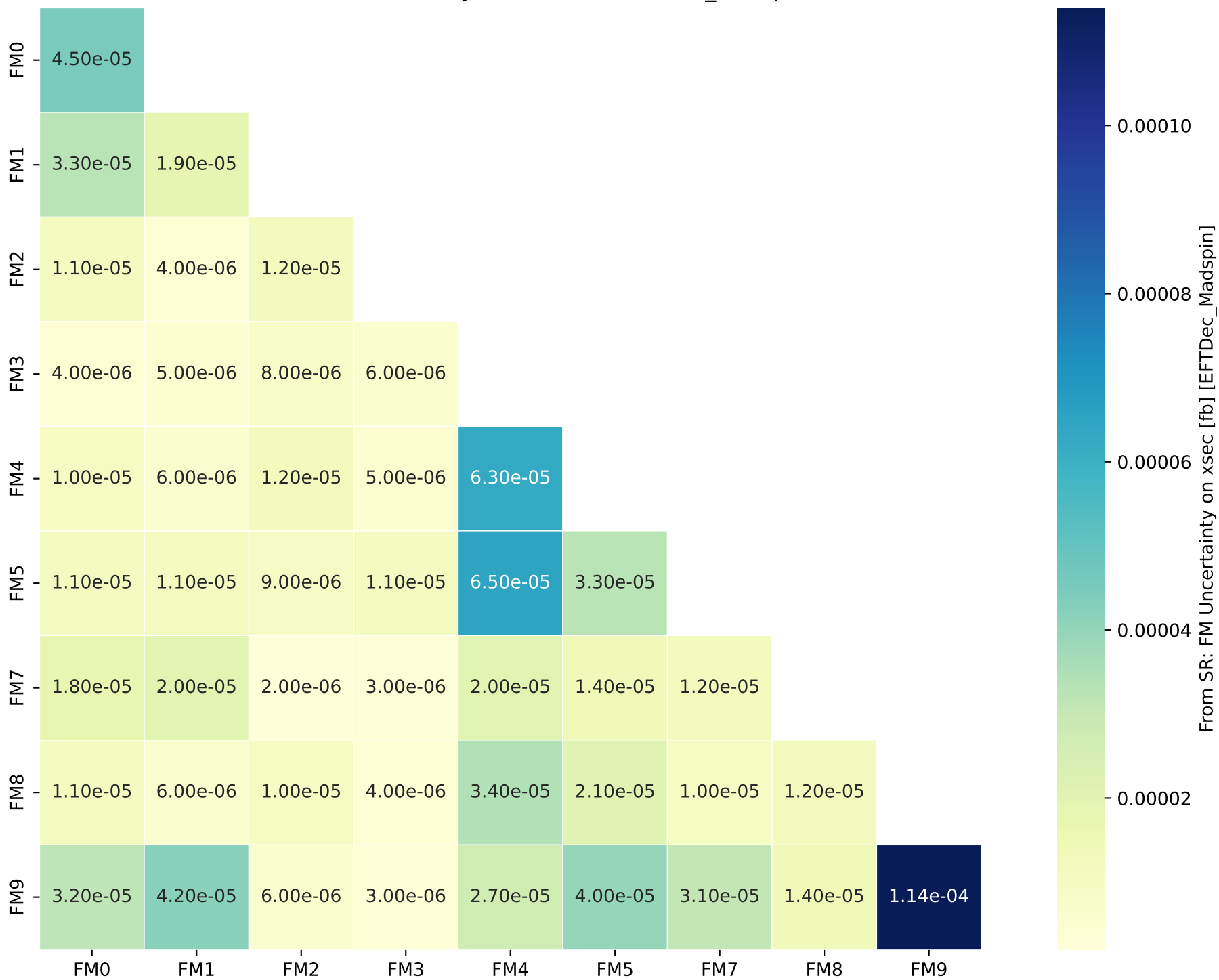
From SR: FM Uncertainty on xsec [fb] [EFTDec_Madspin]
