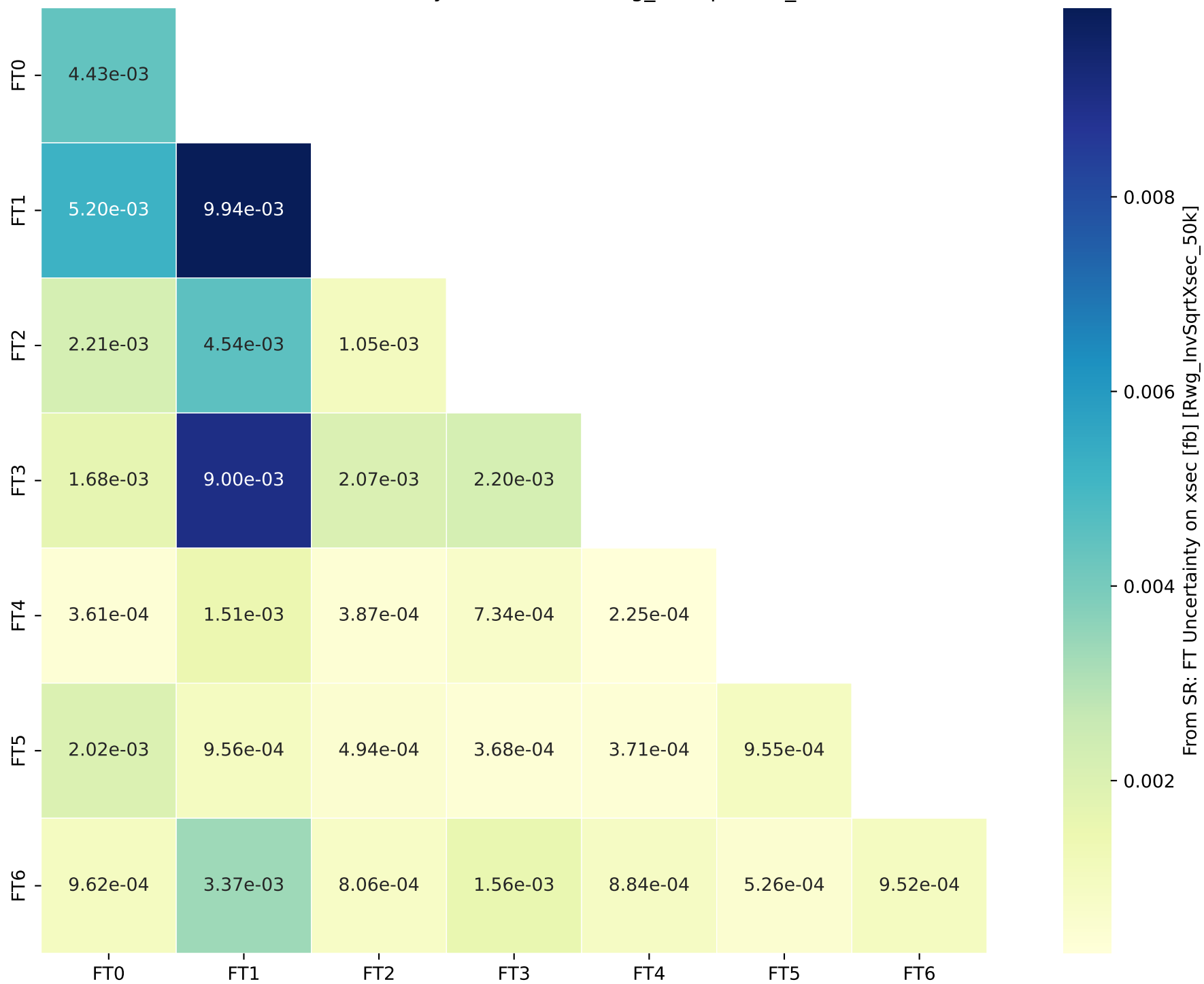
From SR: FT Uncertainty on xsec [fb] [Rwg_InvSqrtXsec_50k]
