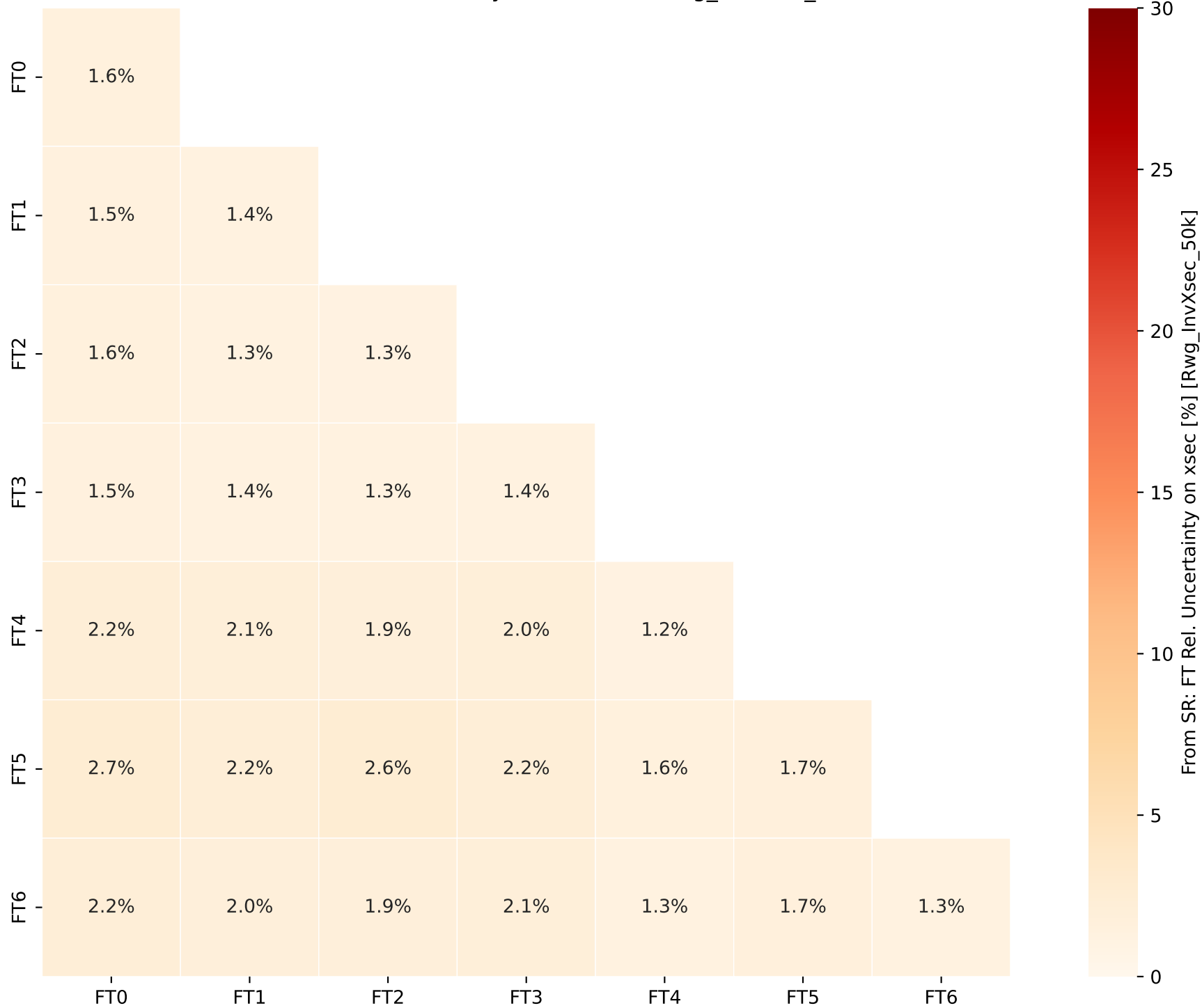
From SR: FT Rel. Uncertainty on xsec [%] [Rwg_InvXsec_50k]
