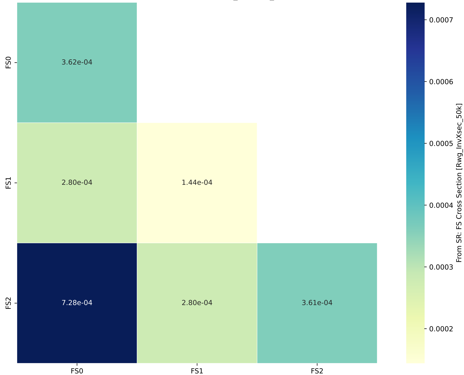
From SR: FS Cross Section [Rwg_InvXsec_50k]
