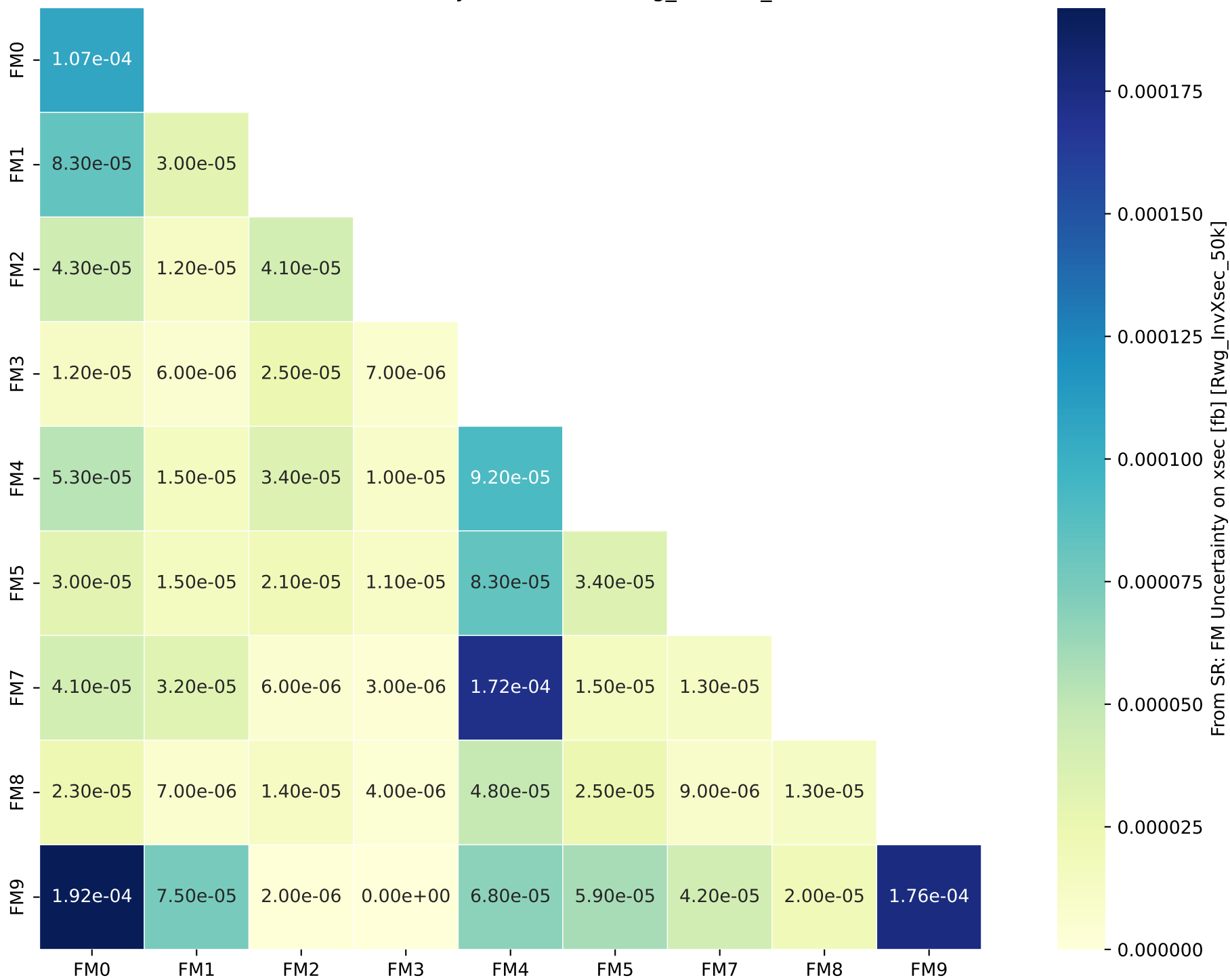
From SR: FM Uncertainty on xsec [fb] [Rwg_InvXsec_50k]
