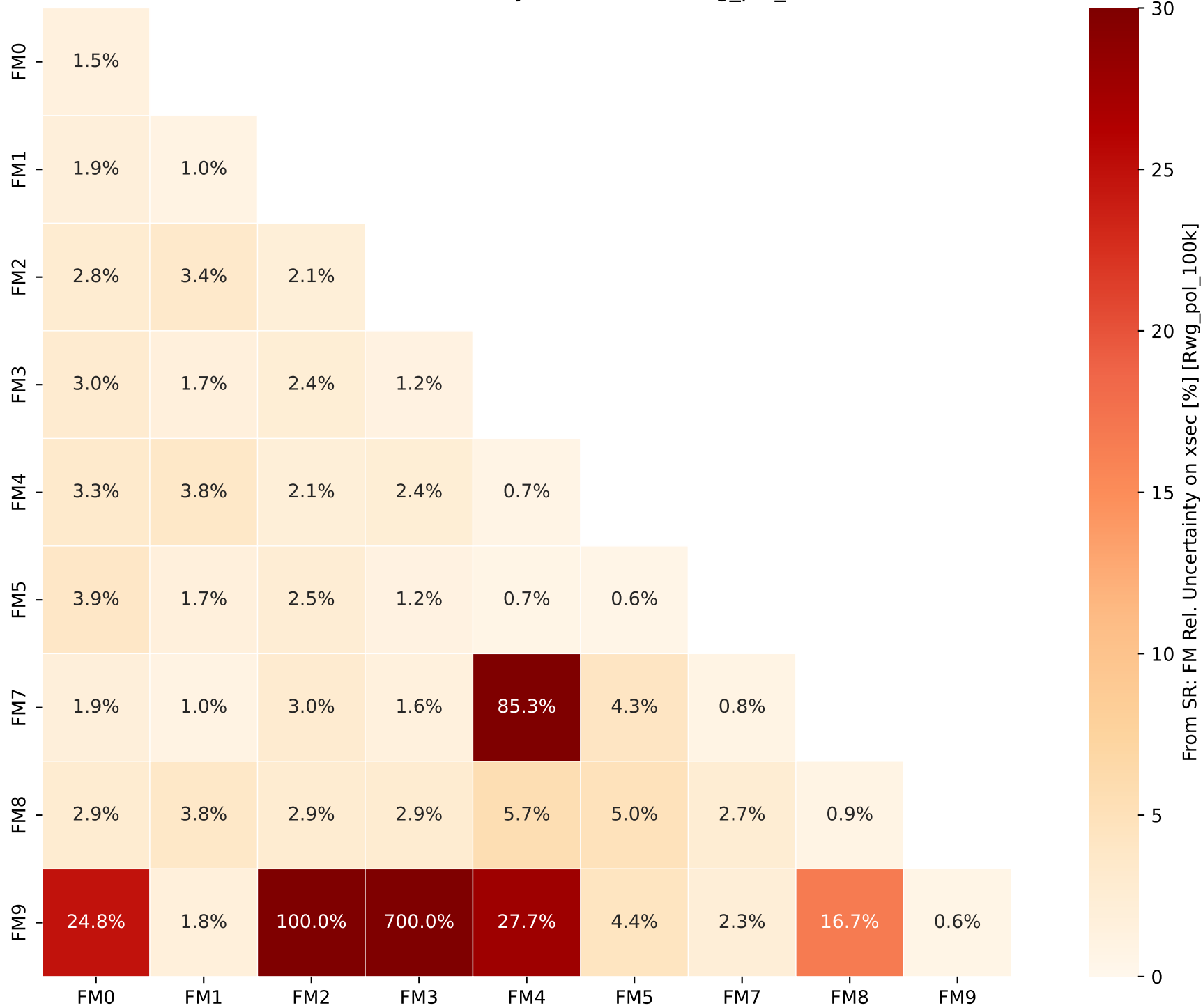
From SR: FM Rel. Uncertainty on xsec [%] [Rwg_pol_100k]
