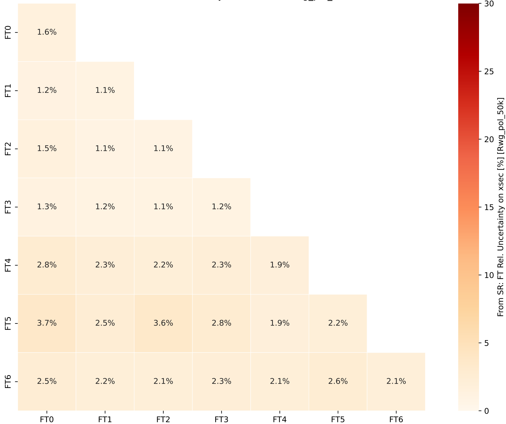
From SR: FT Rel. Uncertainty on xsec [%] [Rwg_pol_50k]
