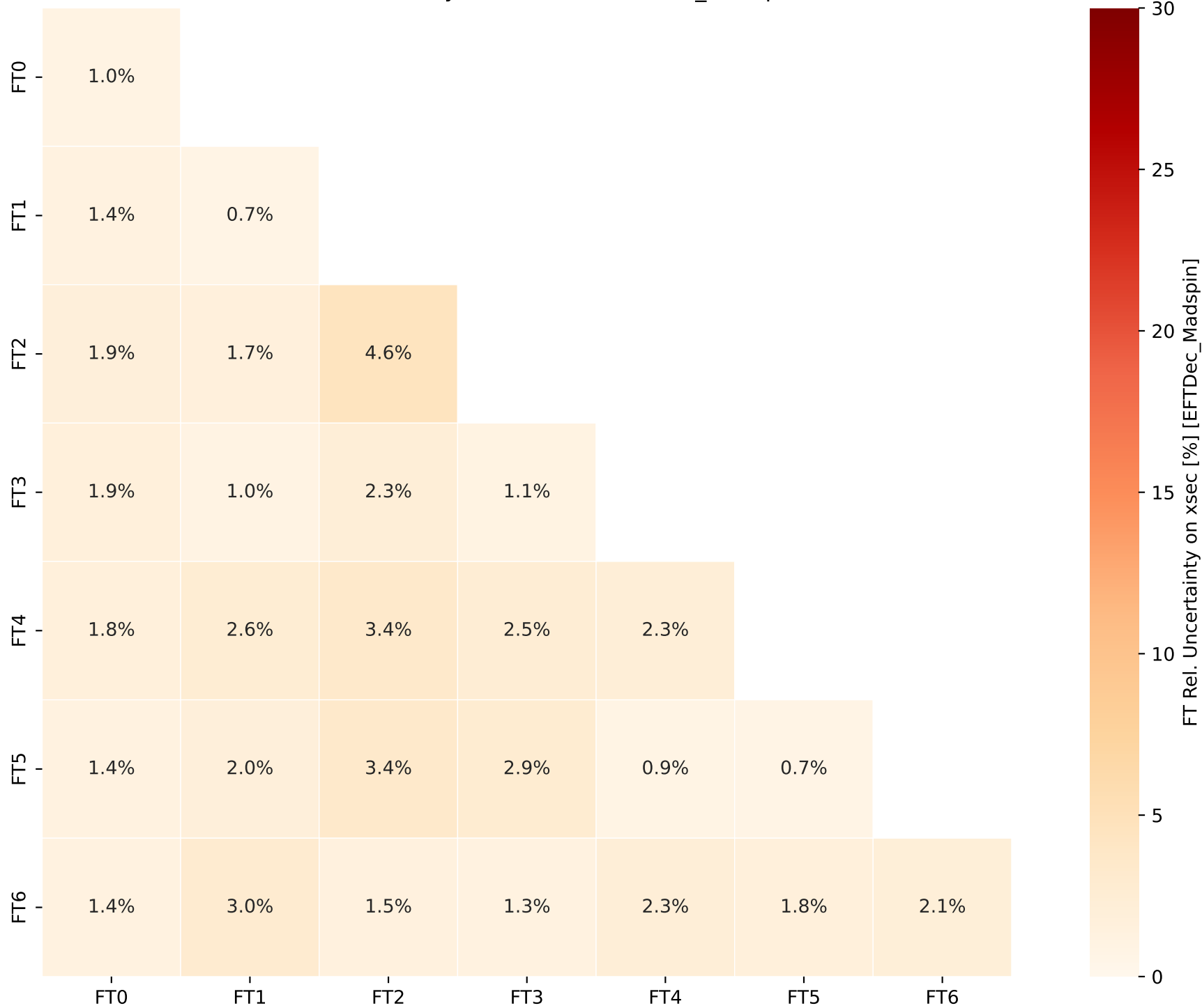
FT Rel. Uncertainty on xsec [%] [EFTDec_Madspin]
