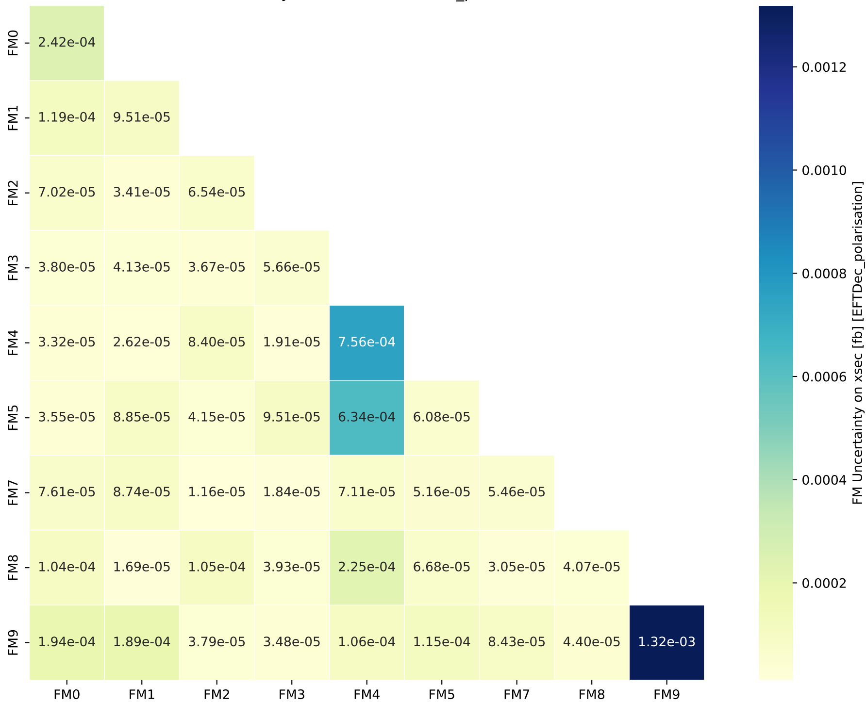
FM Uncertainty on xsec [fb] [EFTDec_polarisation]
