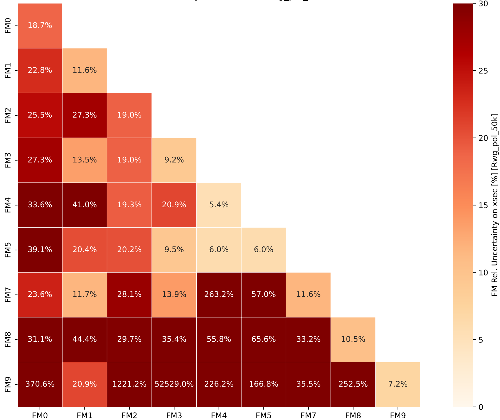
FM Rel. Uncertainty on xsec [%] [Rwg_pol_50k]
