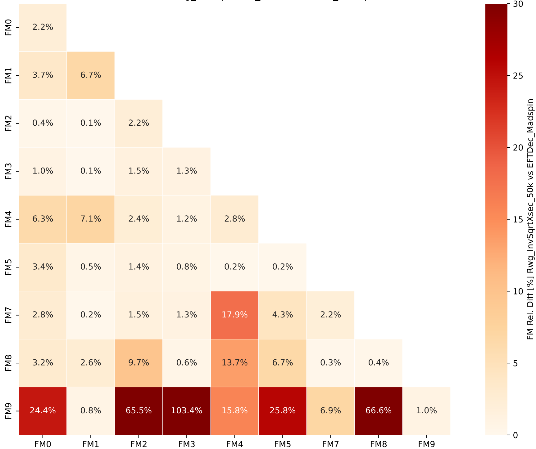
FM Rel. Diff [%] Rwg_InvSqrtXsec_50k vs EFTDec_Madspin
