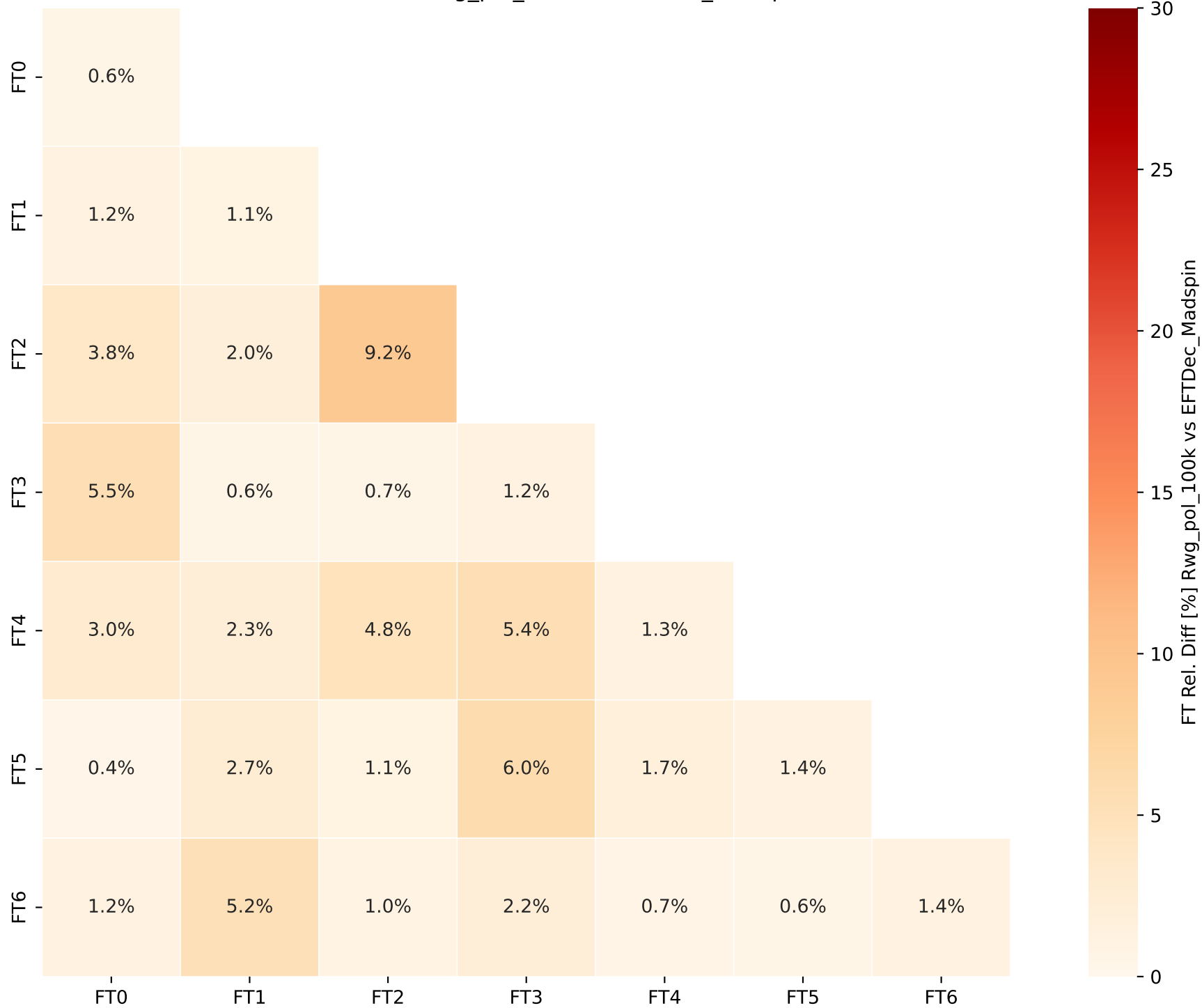
FT Rel. Diff [%] Rwg_pol_100k vs EFTDec_Madspin
