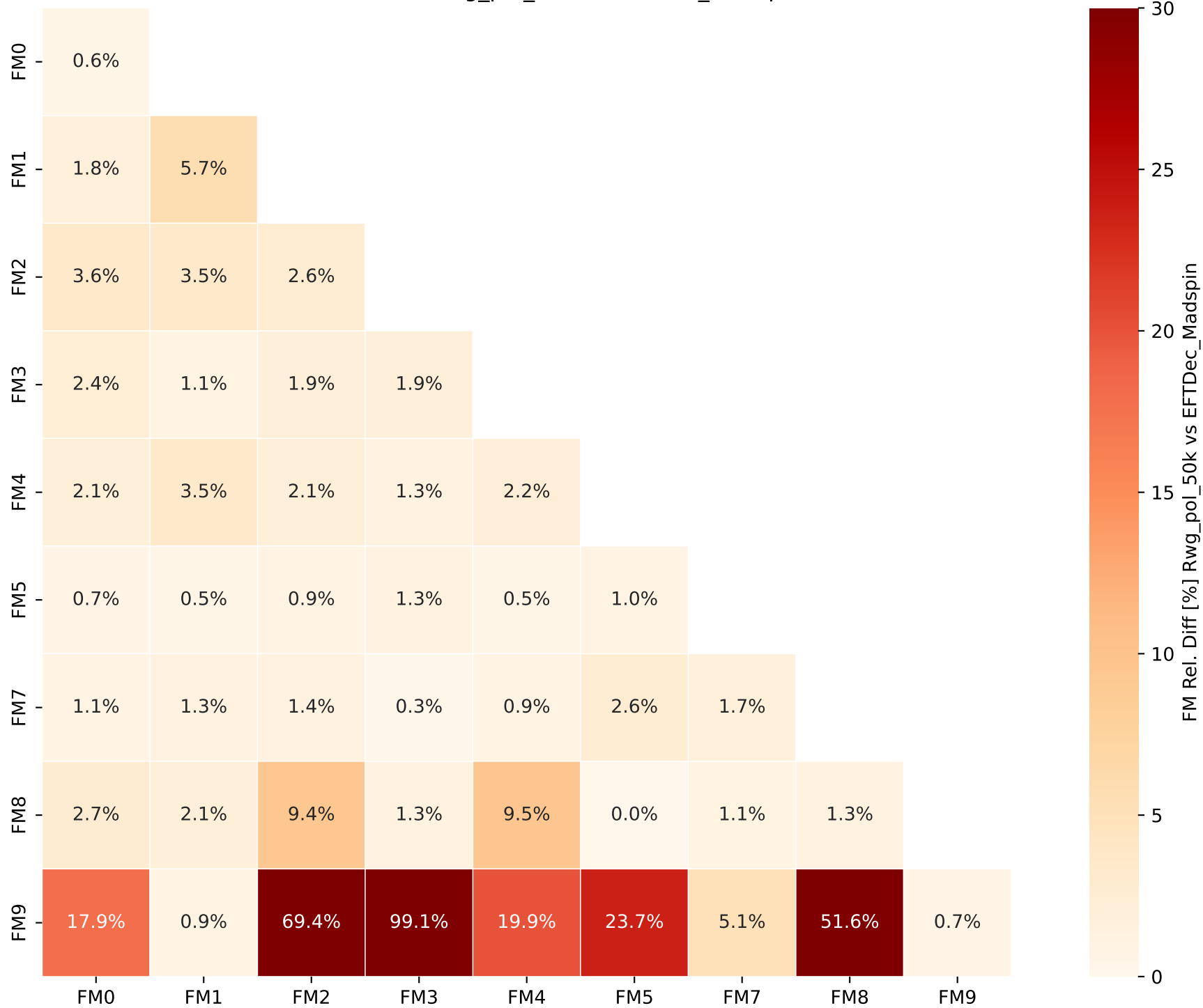
FM Rel. Diff [%] Rwg_pol_50k vs EFTDec_Madspin
