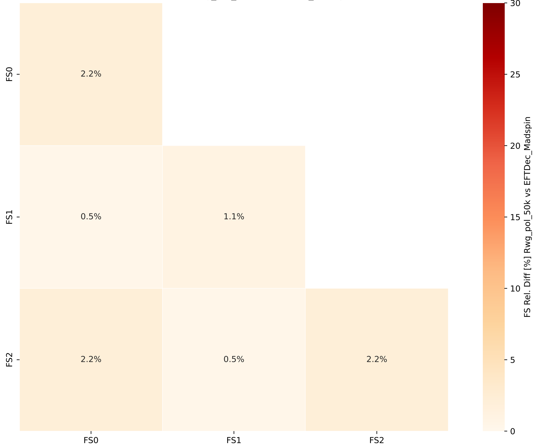
FS Rel. Diff [%] Rwg_pol_50k vs EFTDec_Madspin
