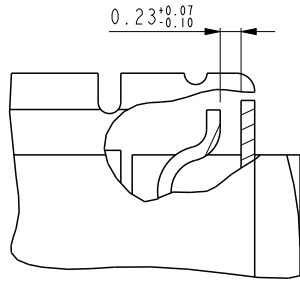
DETAIL C SCALE 12.000
