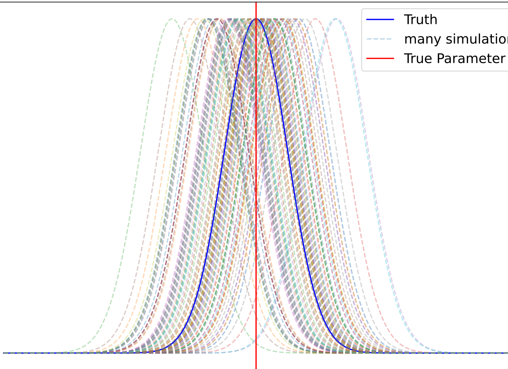
Repetitive MCMC simulations, different noise realisations
