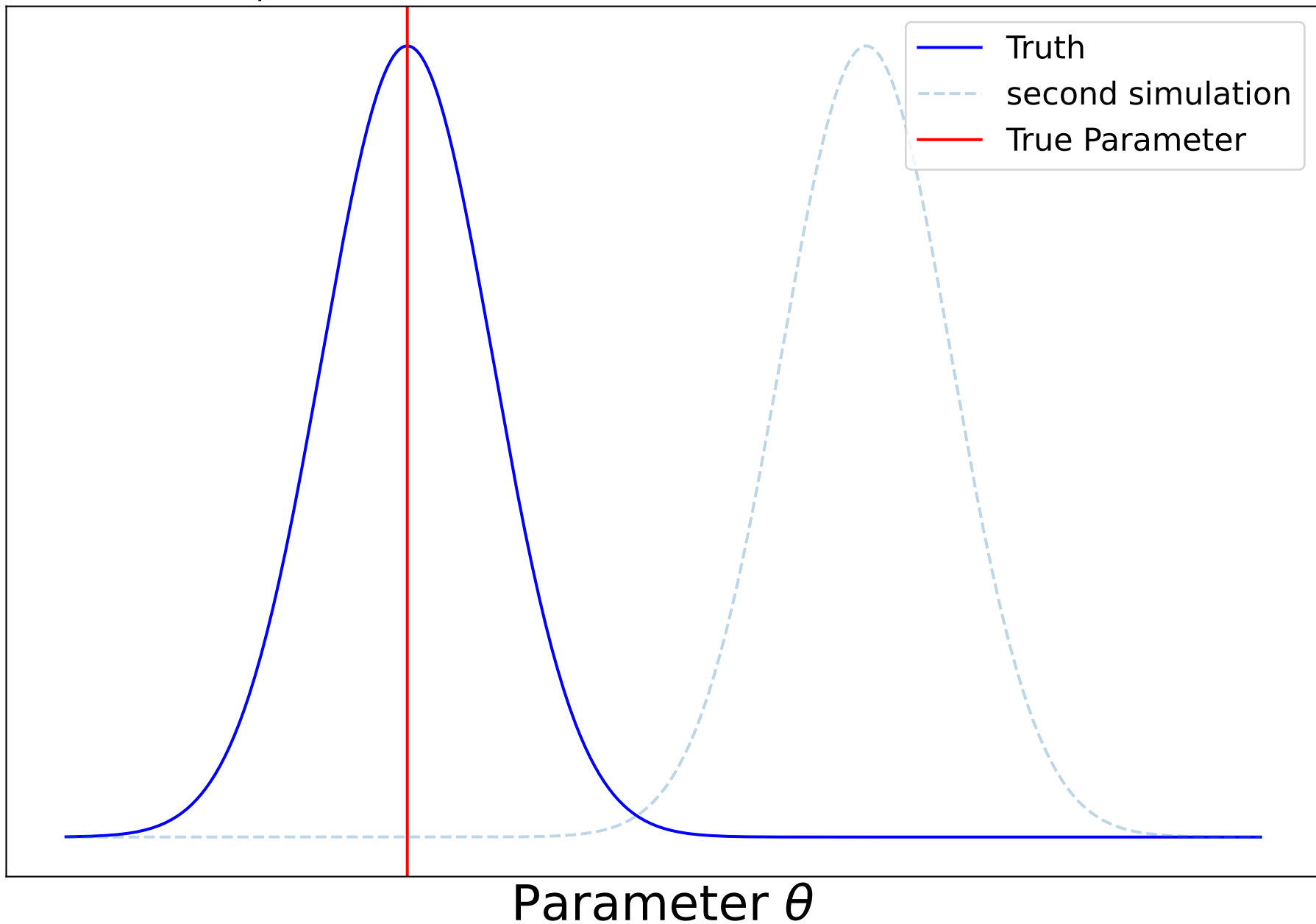
Repetitive MCMC simulations, different noise realisations
