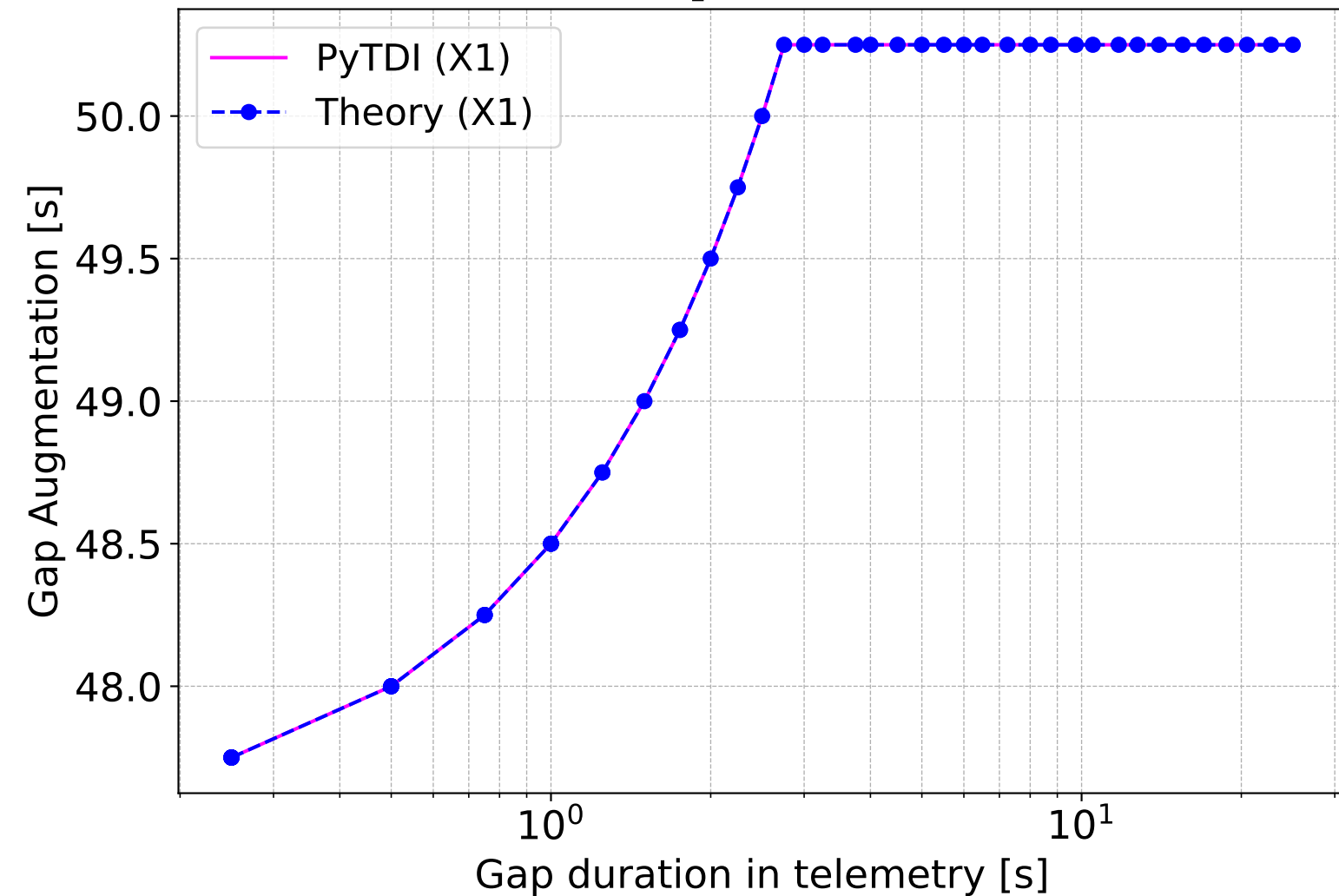
Michelson TDI \mathbf{X}_1 [ \mathcal{K} = 45, \bar{L} = 2.5 \times 10^9 ]
