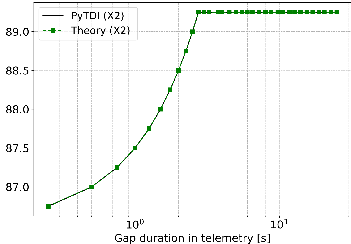
Michelson TDI: \mathbf{X}_2 [ \mathcal{K} = 45, \bar{L} = 2.5 \times 10^9 ]
