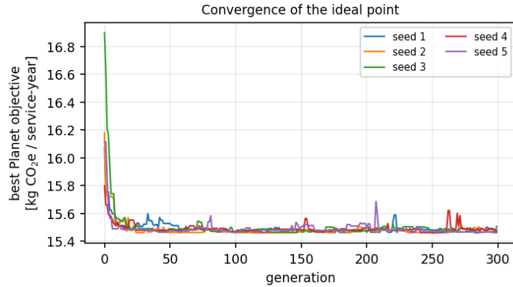
Figure 3: Ideal-point convergence across seeds.
