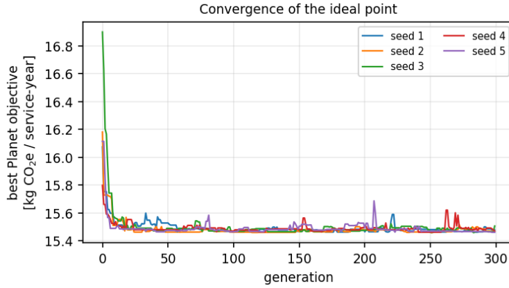
Figure 4: Ideal-point convergence across seeds.
