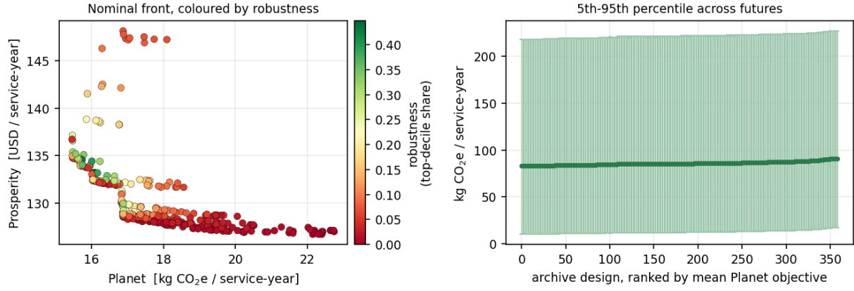
Figure 5: Left: the nominal front coloured by robustness — note that the cheapest nominal designs are not the most robust. Right: 5th–95th percentile spread of the Planet objective across futures, which is dominated by grid decarbonisation and charging-throughput uncertainty.
