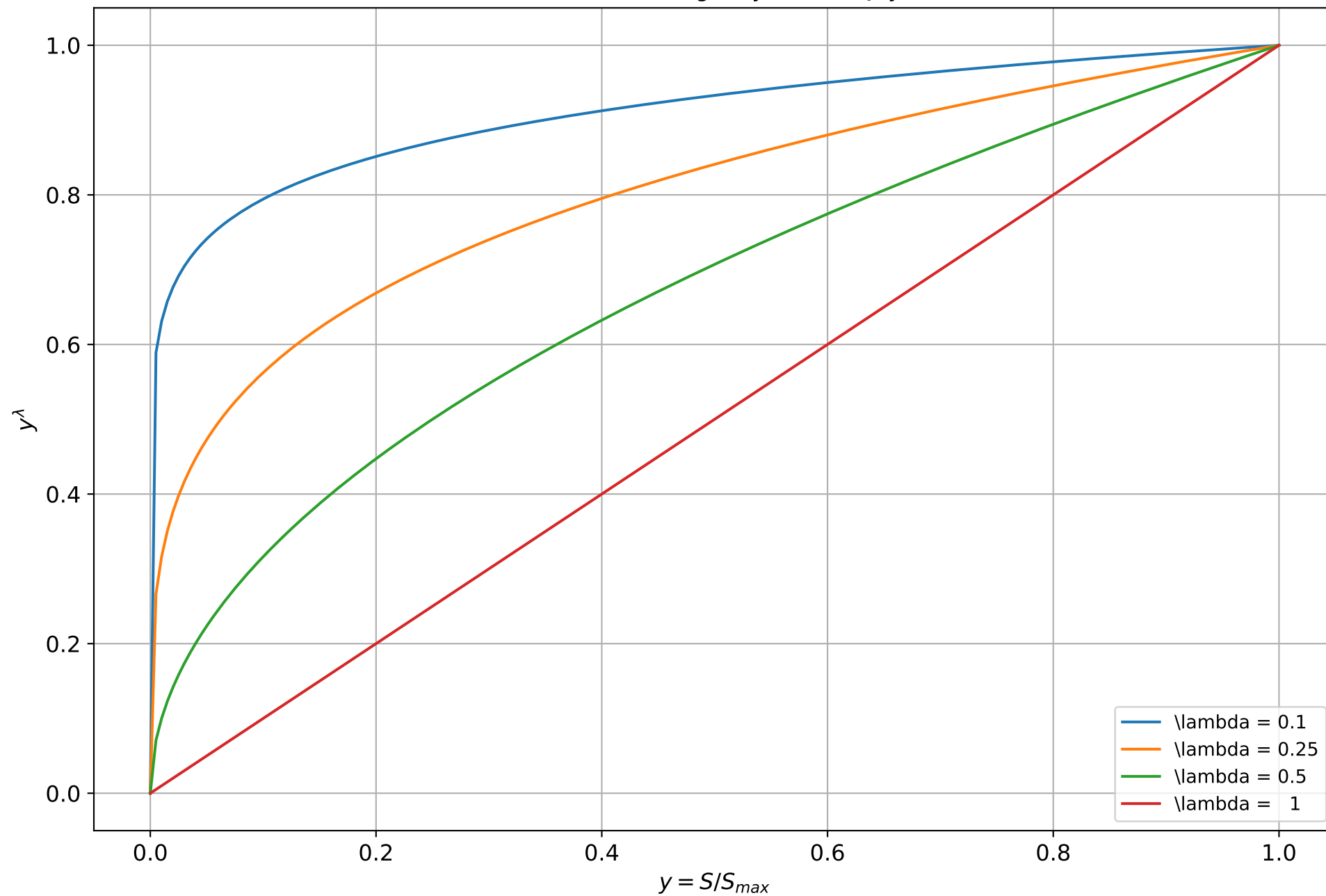
Effect of throttling E by \lambda : ( E = E_0 \cdot y^\lambda )
