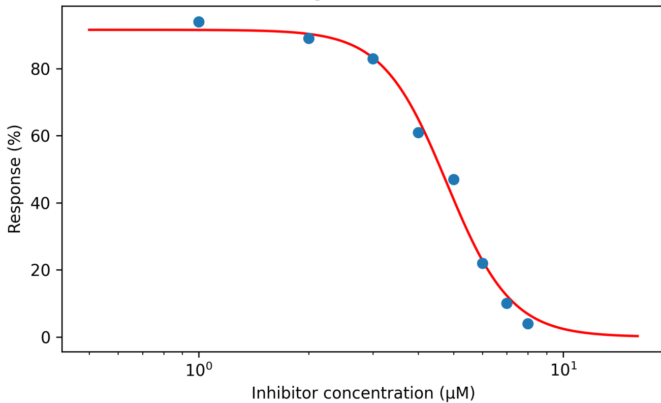
DrugC IC50 Curve
