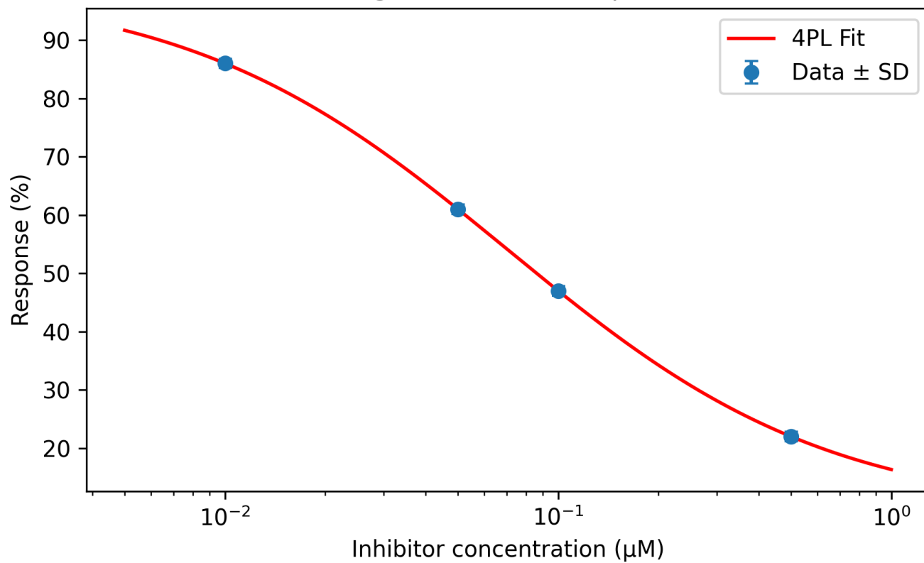
DrugC IC50 Dose-Response
