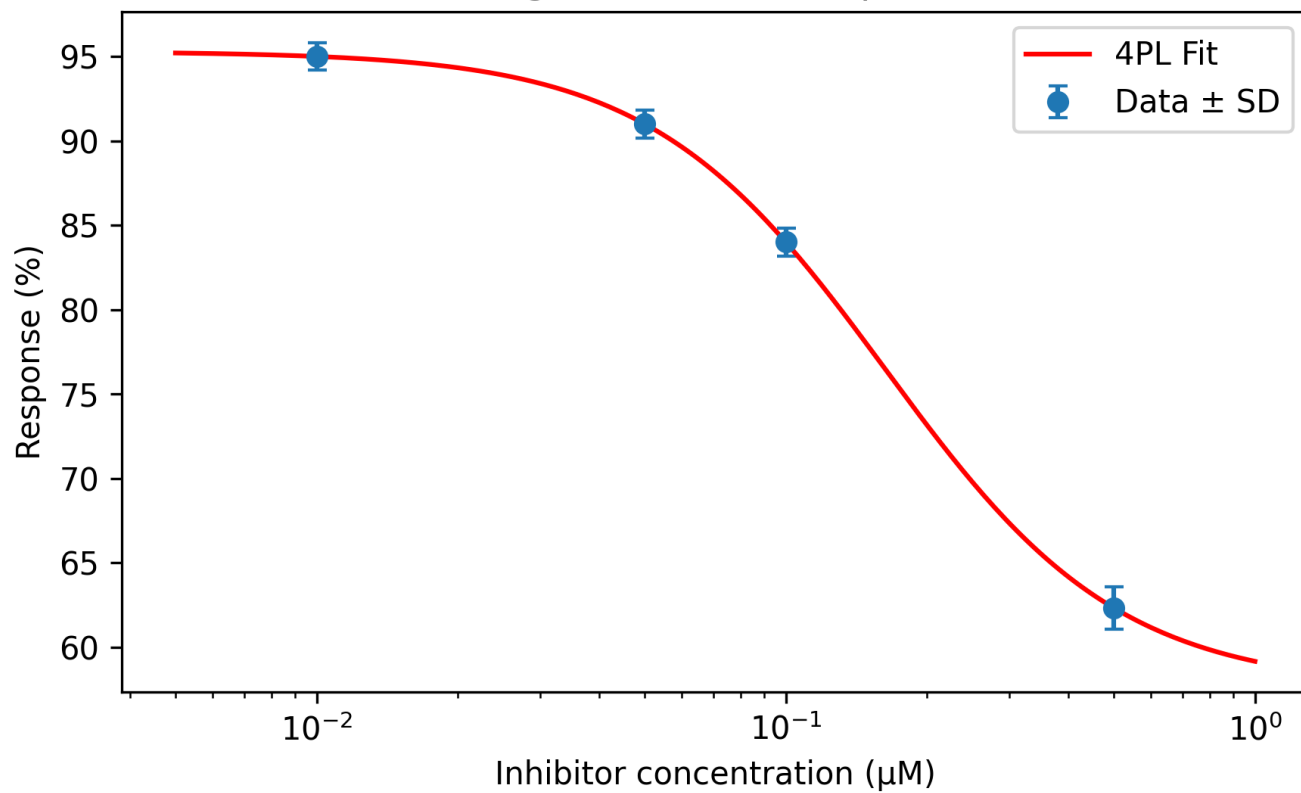
DrugA IC50 Dose-Response
