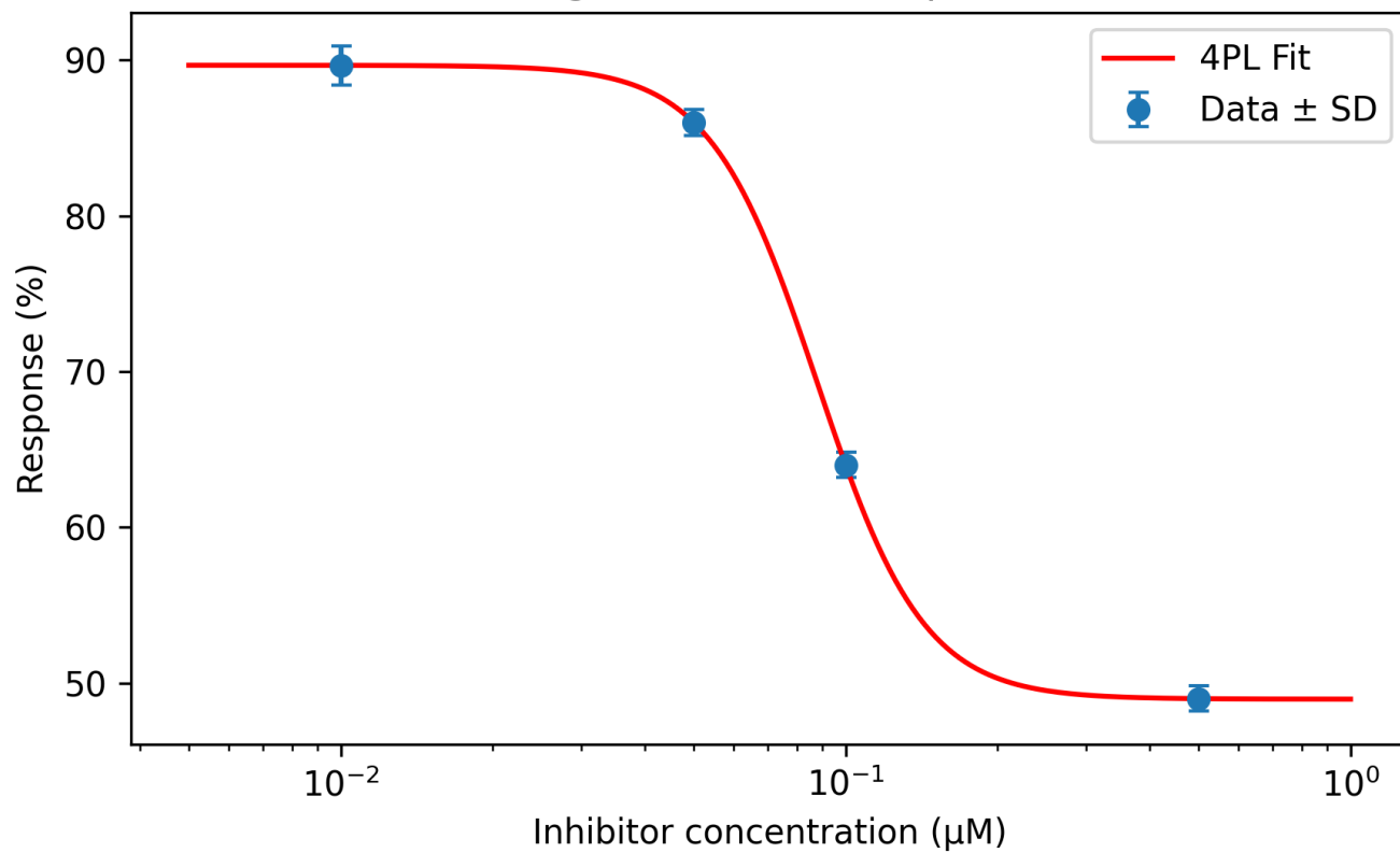
DrugB IC50 Dose-Response
