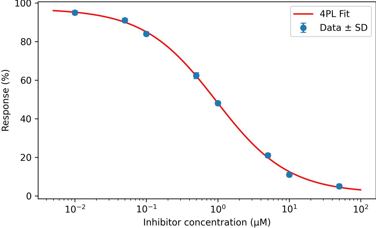
IC50 Dose-Response Curve
