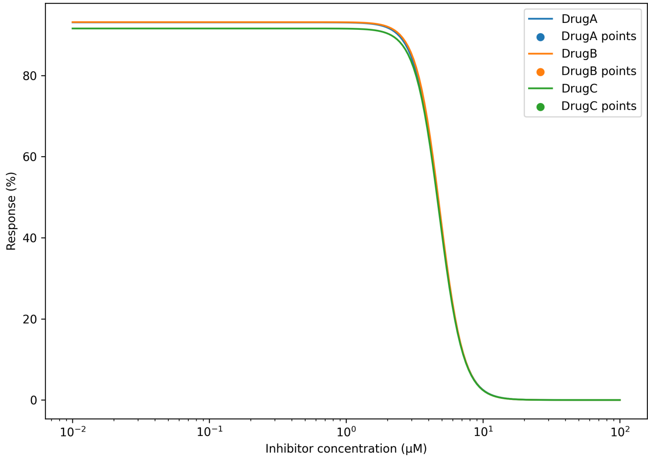
Batch IC50 Dose-Response Curves
