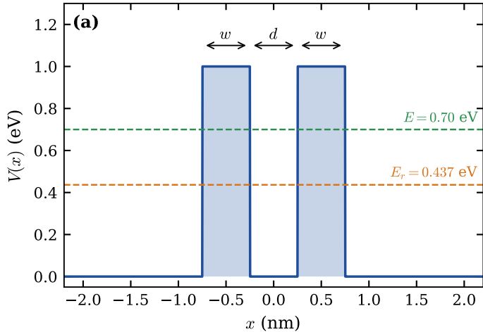
Double barrier: V_0 = 1 eV, w = d = 0.5 nm
