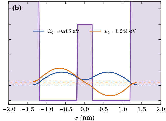
Double well: V_b = 1 eV, b = 0.4 nm, a = 1.0 nm
