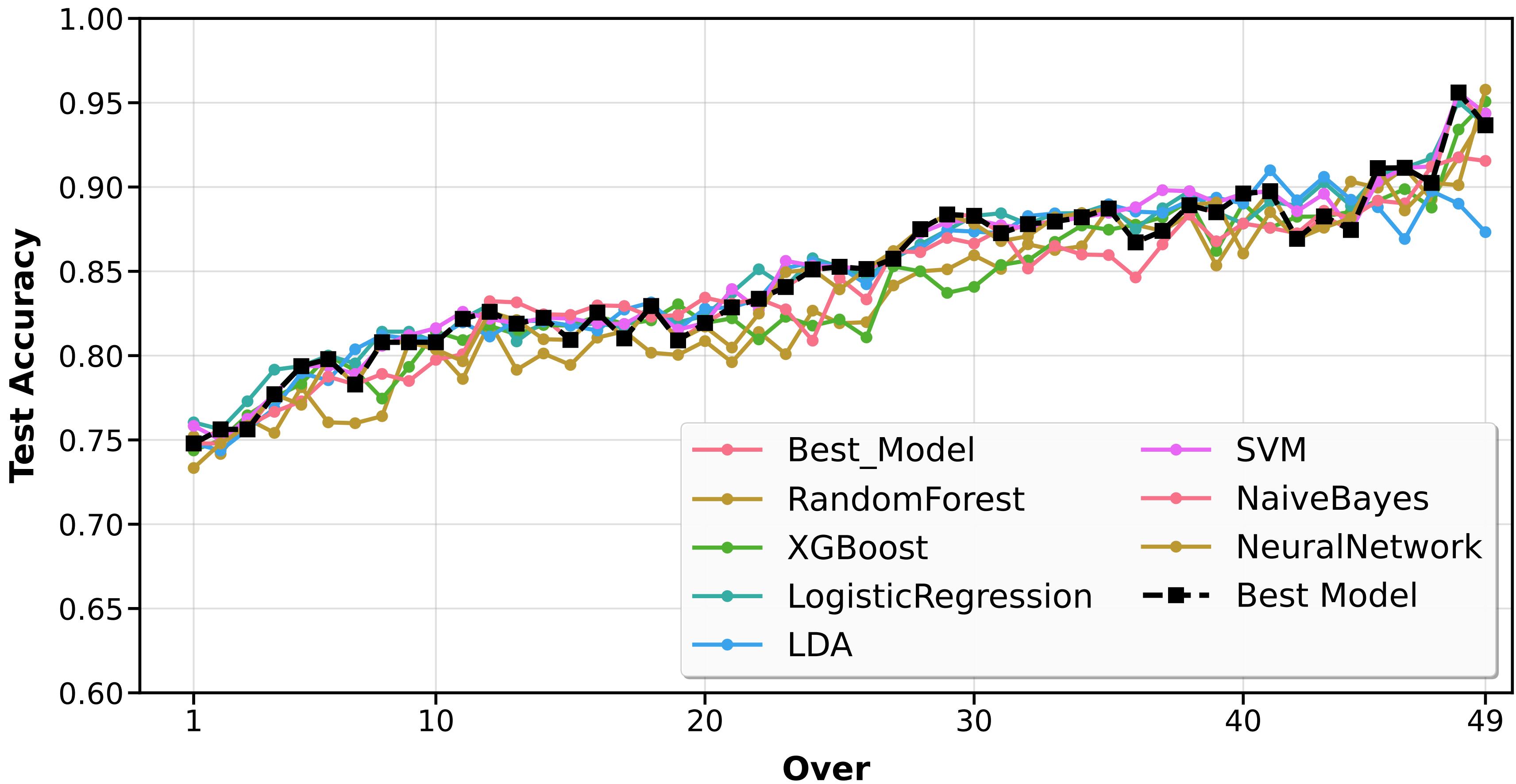
Test Accuracies Across Overs
