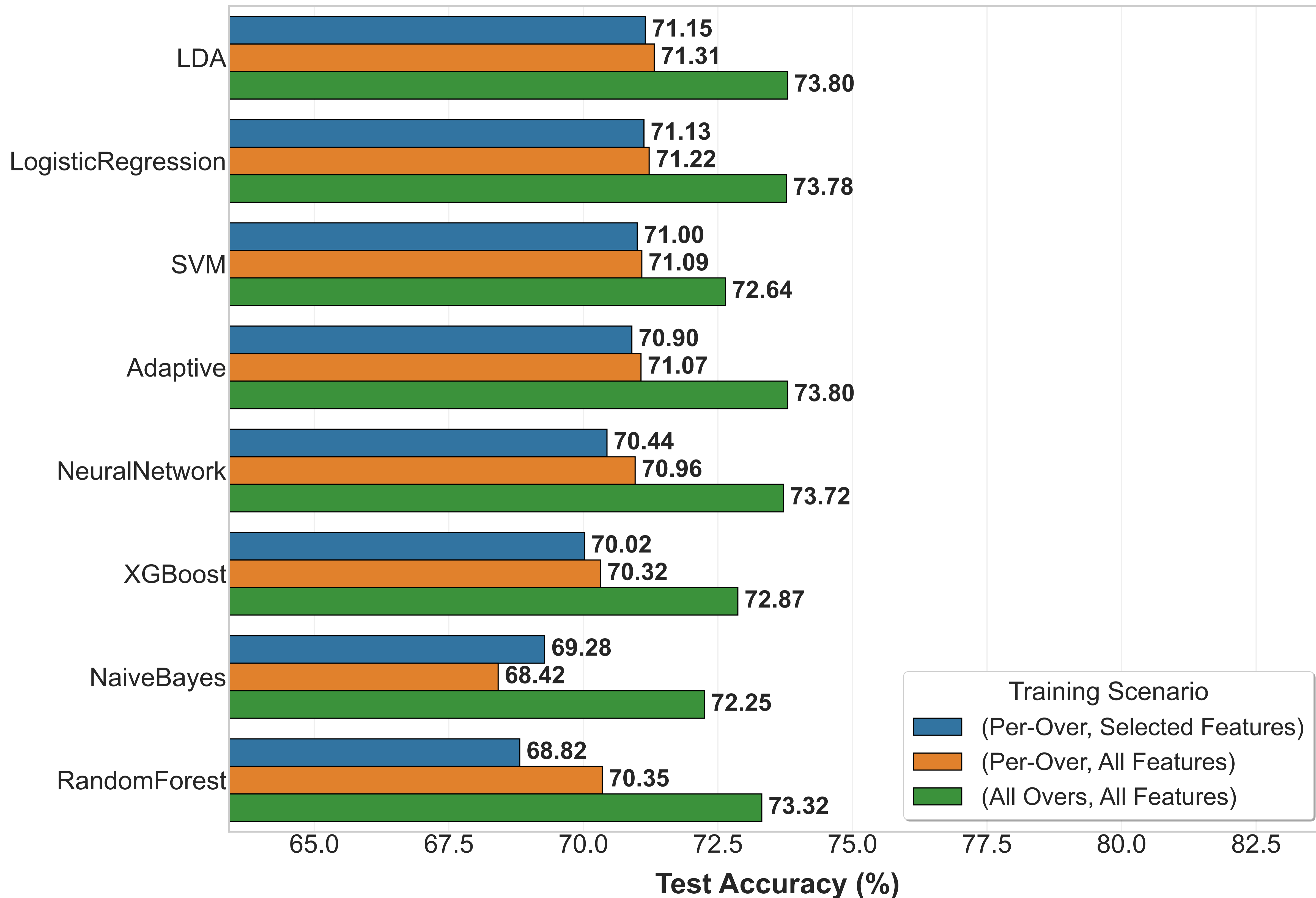
Innings 1: Test Accuracy Comparison
