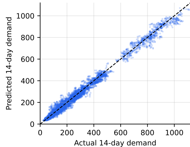
LightGBM WMAPE = 6.77%
