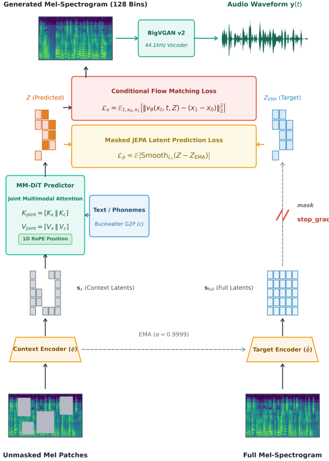
Fig. 1. The Fusion-JEPA multimodal architecture. Phoneme text tokens and audio spectrogram patches are processed jointly through MM-DiT blocks with 1D RoPE, supervised simultaneously by a Flow Matching velocity loss ( \mathcal{L}_v ) and a JEPA latent prediction loss ( \mathcal{L}_p ).
