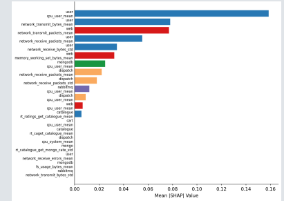
Figure 3: Top 20 SHAP feature Importances
