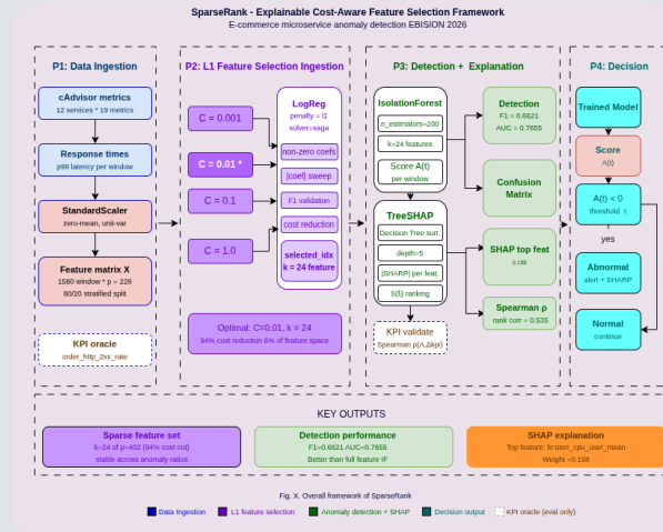
Figure 1: Overall framework of SparseRank.
