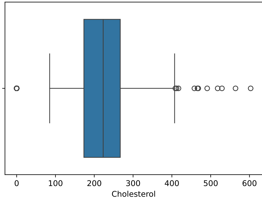
Cholesterol Boxplot
