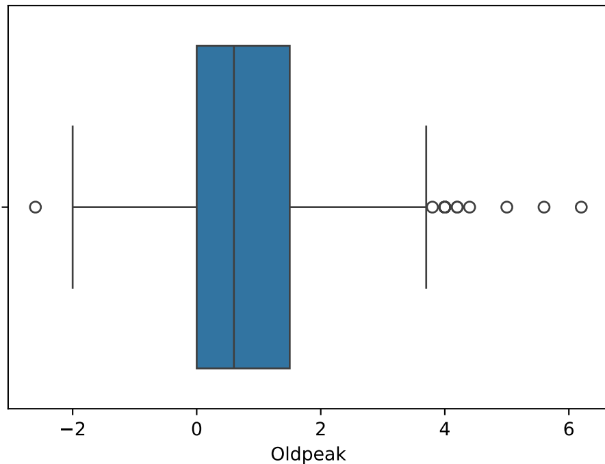
Oldpeak Boxplot
