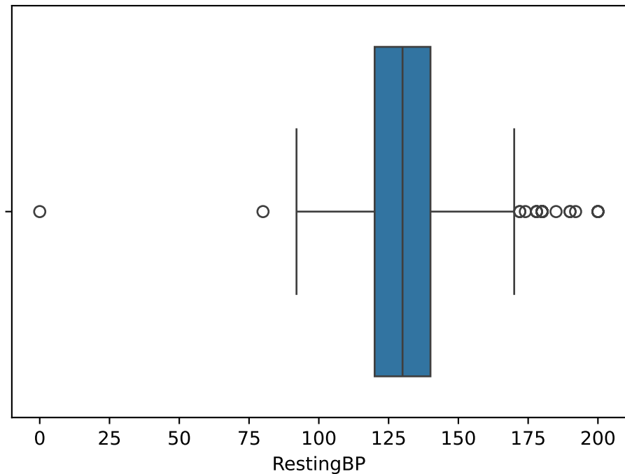
RestingBP Boxplot
