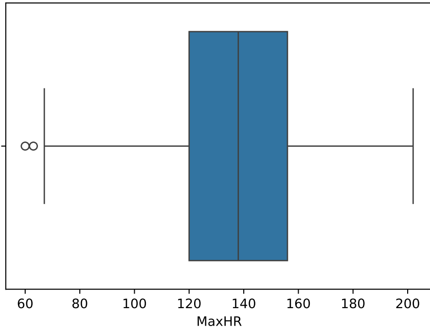
MaxHR Boxplot
