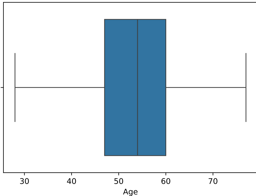
Age Boxplot
