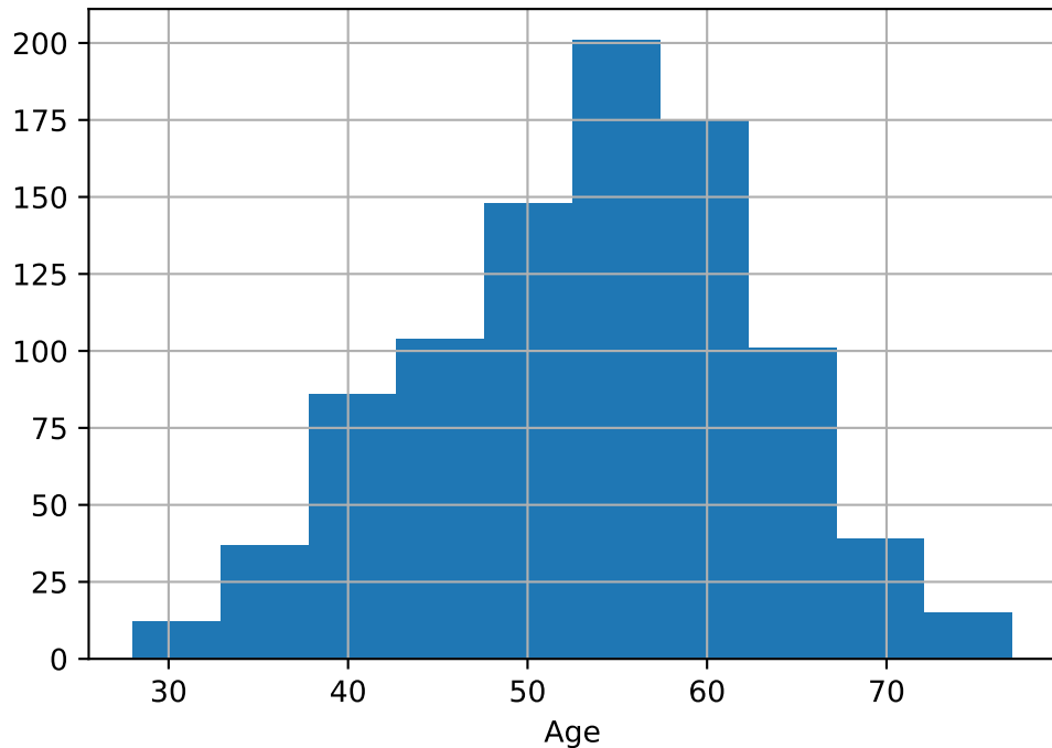
Age Histogram
