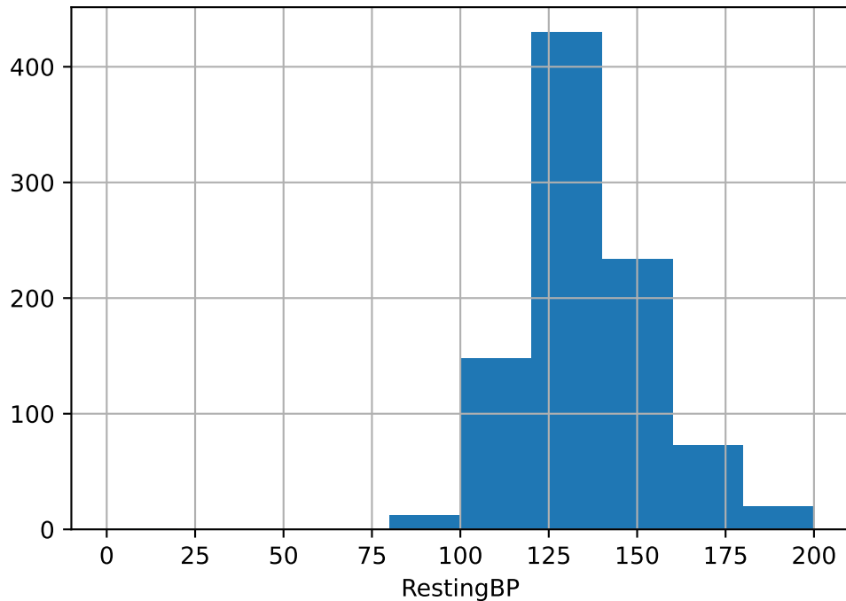
RestingBP Histogram
