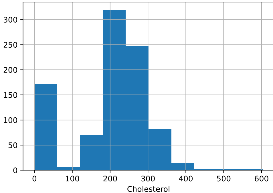
Cholesterol Histogram
