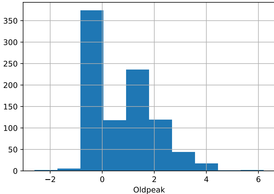
Oldpeak Histogram
